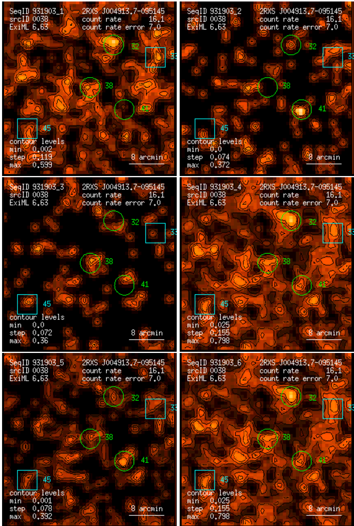
Figure 38: RASS 931903: detection 0038: band rate images, Gaussian filter: (1) PSPC channels 11 – 41, (2) 52 – 90, (3) 91 – 201, (4) 11 – 235, (5) 52 – 201, (6) 11 – 201. Broad band rates in counts/ks. Band rate contour levels in counts/ks/arcmin 2 .
