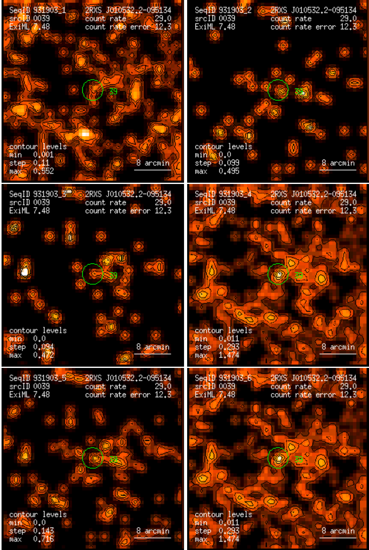
Figure 39: RASS 931903: detection 0039: band rate images, Gaussian filter: (1) PSPC channels 11 – 41, (2) 52 – 90, (3) 91 – 201, (4) 11 – 235, (5) 52 – 201, (6) 11 – 201. Broad band rates in counts/ks. Band rate contour levels in counts/ks/arcmin 2 .
