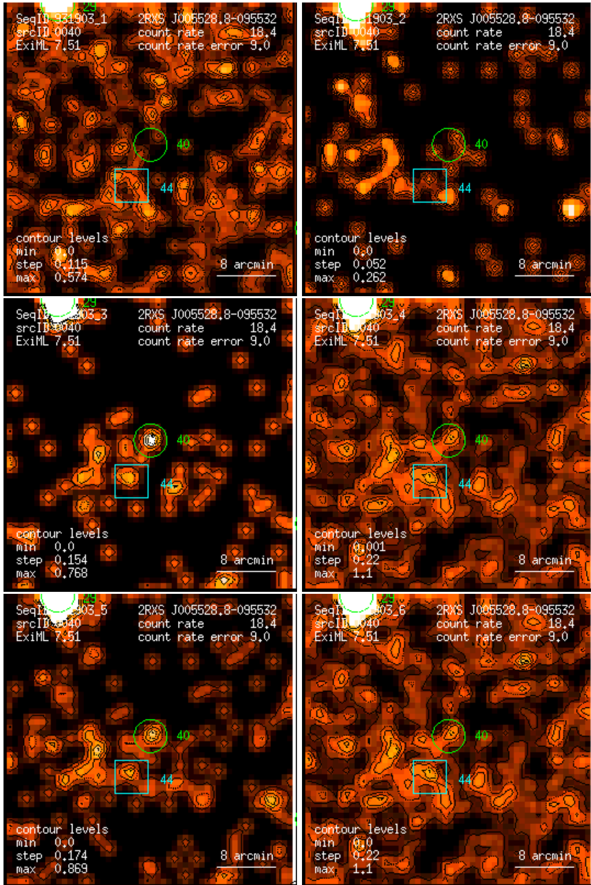
Figure 40: RASS 931903: detection 0040: band rate images, Gaussian filter: (1) PSPC channels 11 – 41, (2) 52 – 90, (3) 91 – 201, (4) 11 – 235, (5) 52 – 201, (6) 11 – 201. Broad band rates in counts/ks. Band rate contour levels in counts/ks/arcmin 2 .
