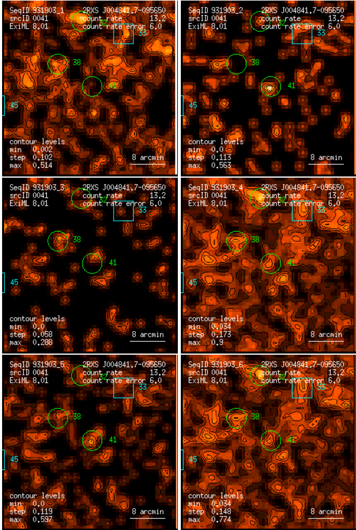
Figure 41: RASS 931903: detection 0041: band rate images, Gaussian filter: (1) PSPC channels 11 – 41, (2) 52 – 90, (3) 91 – 201, (4) 11 – 235, (5) 52 – 201, (6) 11 – 201. Broad band rates in counts/ks. Band rate contour levels in counts/ks/arcmin 2 .
