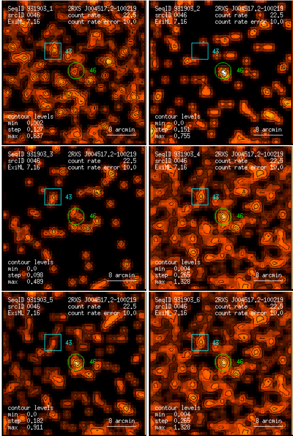
Figure 46: RASS 931903: detection 0046: band rate images, Gaussian filter: (1) PSPC channels 11 – 41, (2) 52 – 90, (3) 91 – 201, (4) 11 – 235, (5) 52 – 201, (6) 11 – 201. Broad band rates in counts/ks. Band rate contour levels in counts/ks/arcmin 2 .
