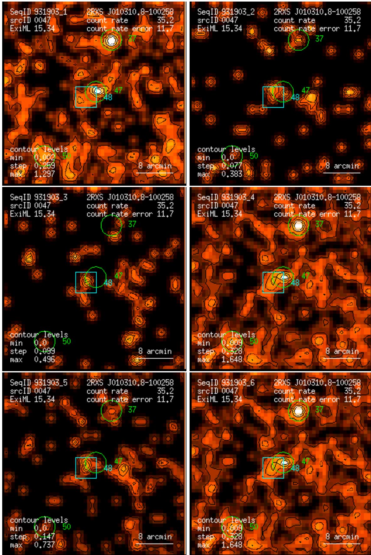
Figure 47: RASS 931903: detection 0047: band rate images, Gaussian filter: (1) PSPC channels 11 – 41, (2) 52 – 90, (3) 91 – 201, (4) 11 – 235, (5) 52 – 201, (6) 11 – 201. Broad band rates in counts/ks. Band rate contour levels in counts/ks/arcmin 2 .
