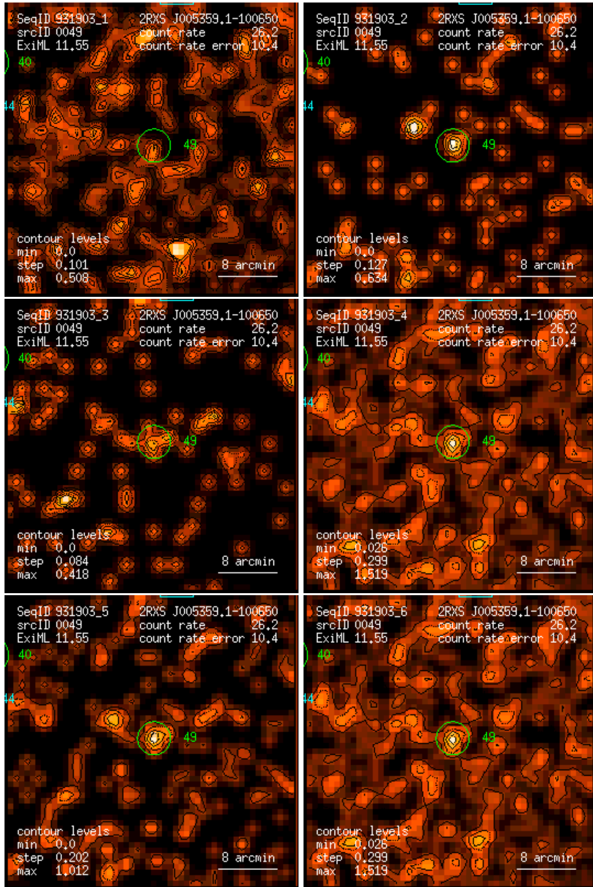
Figure 49: RASS 931903: detection 0049: band rate images, Gaussian filter: (1) PSPC channels 11 – 41, (2) 52 – 90, (3) 91 – 201, (4) 11 – 235, (5) 52 – 201, (6) 11 – 201. Broad band rates in counts/ks. Band rate contour levels in counts/ks/arcmin 2 .
