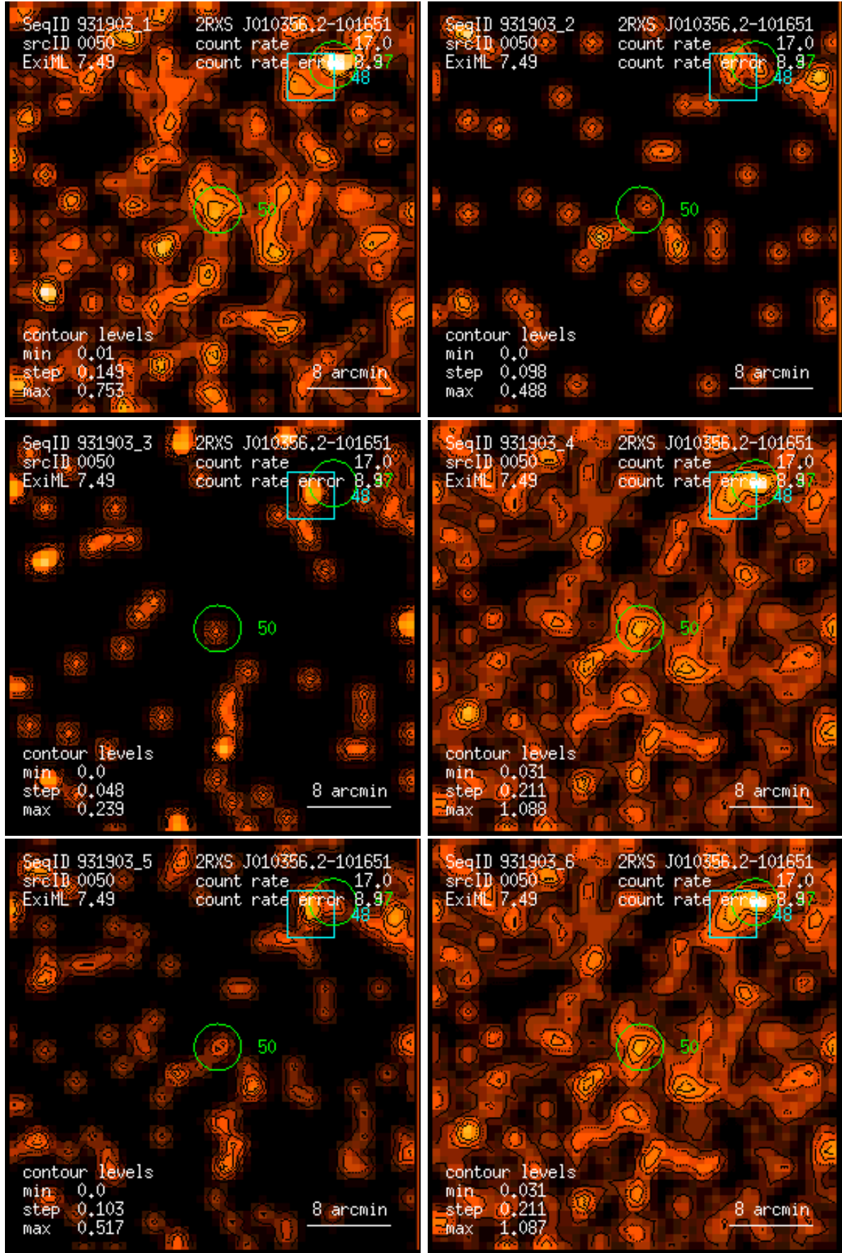
Figure 50: RASS 931903: detection 0050: band rate images, Gaussian filter: (1) PSPC channels 11 – 41, (2) 52 – 90, (3) 91 – 201, (4) 11 – 235, (5) 52 – 201, (6) 11 – 201. Broad band rates in counts/ks. Band rate contour levels in counts/ks/arcmin 2 .
