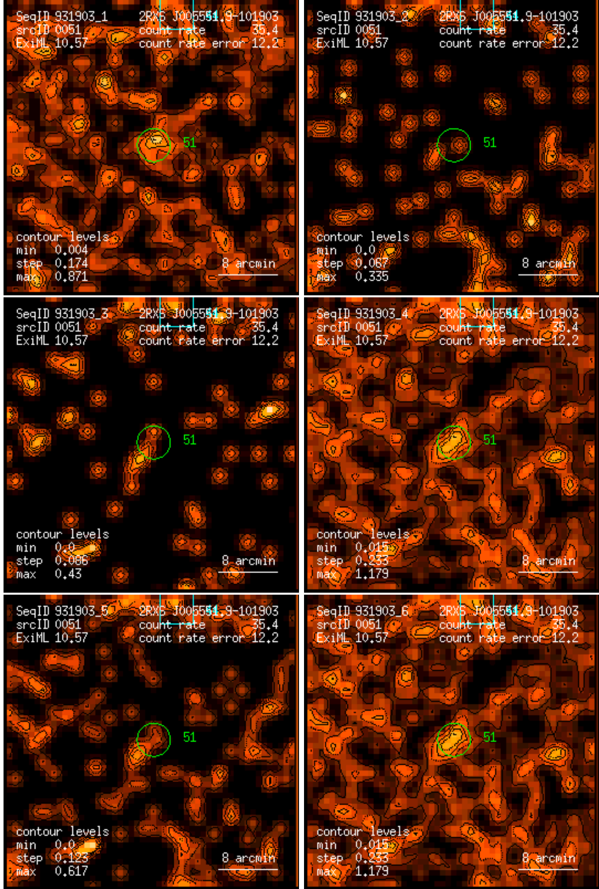
Figure 51: RASS 931903: detection 0051: band rate images, Gaussian filter: (1) PSPC channels 11 – 41, (2) 52 – 90, (3) 91 – 201, (4) 11 – 235, (5) 52 – 201, (6) 11 – 201. Broad band rates in counts/ks. Band rate contour levels in counts/ks/arcmin 2 .
