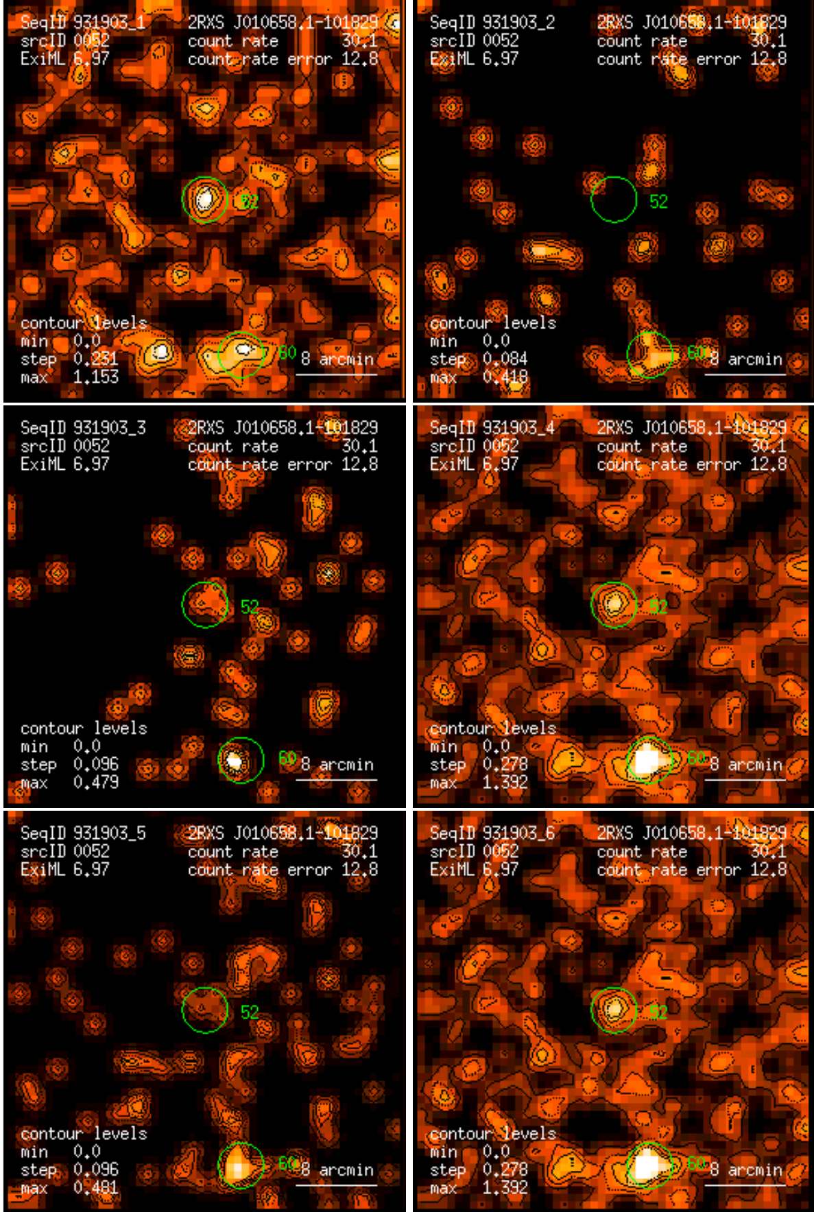
Figure 52: RASS 931903: detection 0052: band rate images, Gaussian filter: (1) PSPC channels 11 – 41, (2) 52 – 90, (3) 91 – 201, (4) 11 – 235, (5) 52 – 201, (6) 11 – 201. Broad band rates in counts/ks. Band rate contour levels in counts/ks/arcmin 2 .
