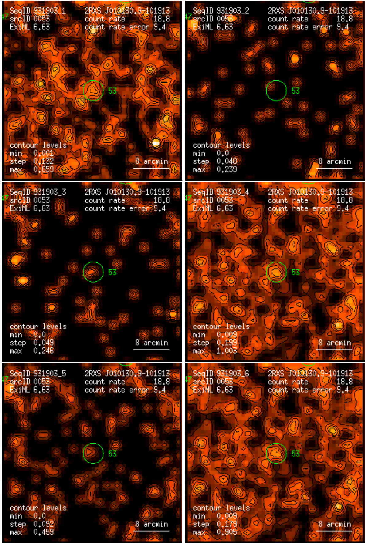
Figure 53: RASS 931903: detection 0053: band rate images, Gaussian filter: (1) PSPC channels 11 – 41, (2) 52 – 90, (3) 91 – 201, (4) 11 – 235, (5) 52 – 201, (6) 11 – 201. Broad band rates in counts/ks. Band rate contour levels in counts/ks/arcmin 2 .
