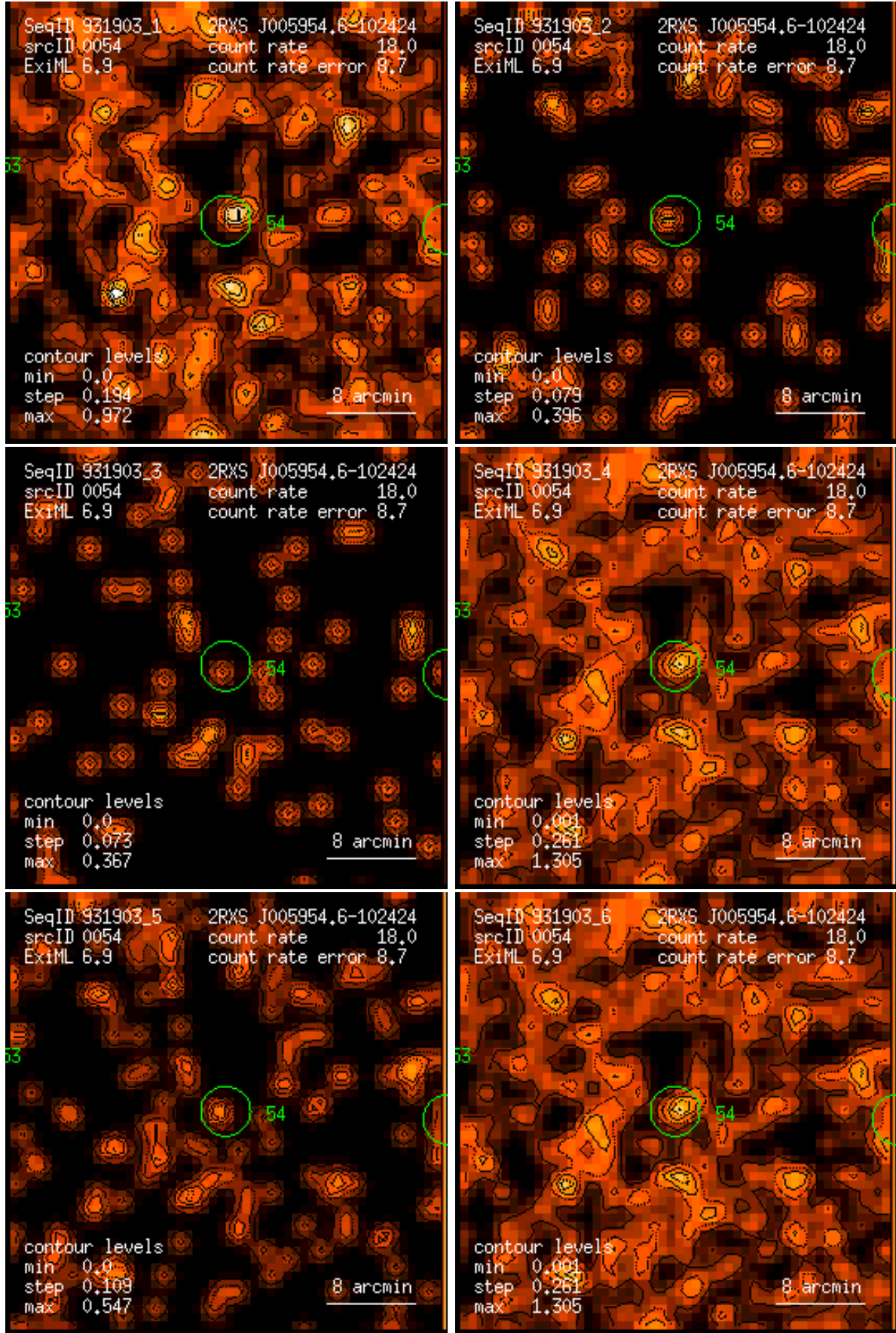
Figure 54: RASS 931903: detection 0054: band rate images, Gaussian filter: (1) PSPC channels 11 – 41, (2) 52 – 90, (3) 91 – 201, (4) 11 – 235, (5) 52 – 201, (6) 11 – 201. Broad band rates in counts/ks. Band rate contour levels in counts/ks/arcmin 2 .
