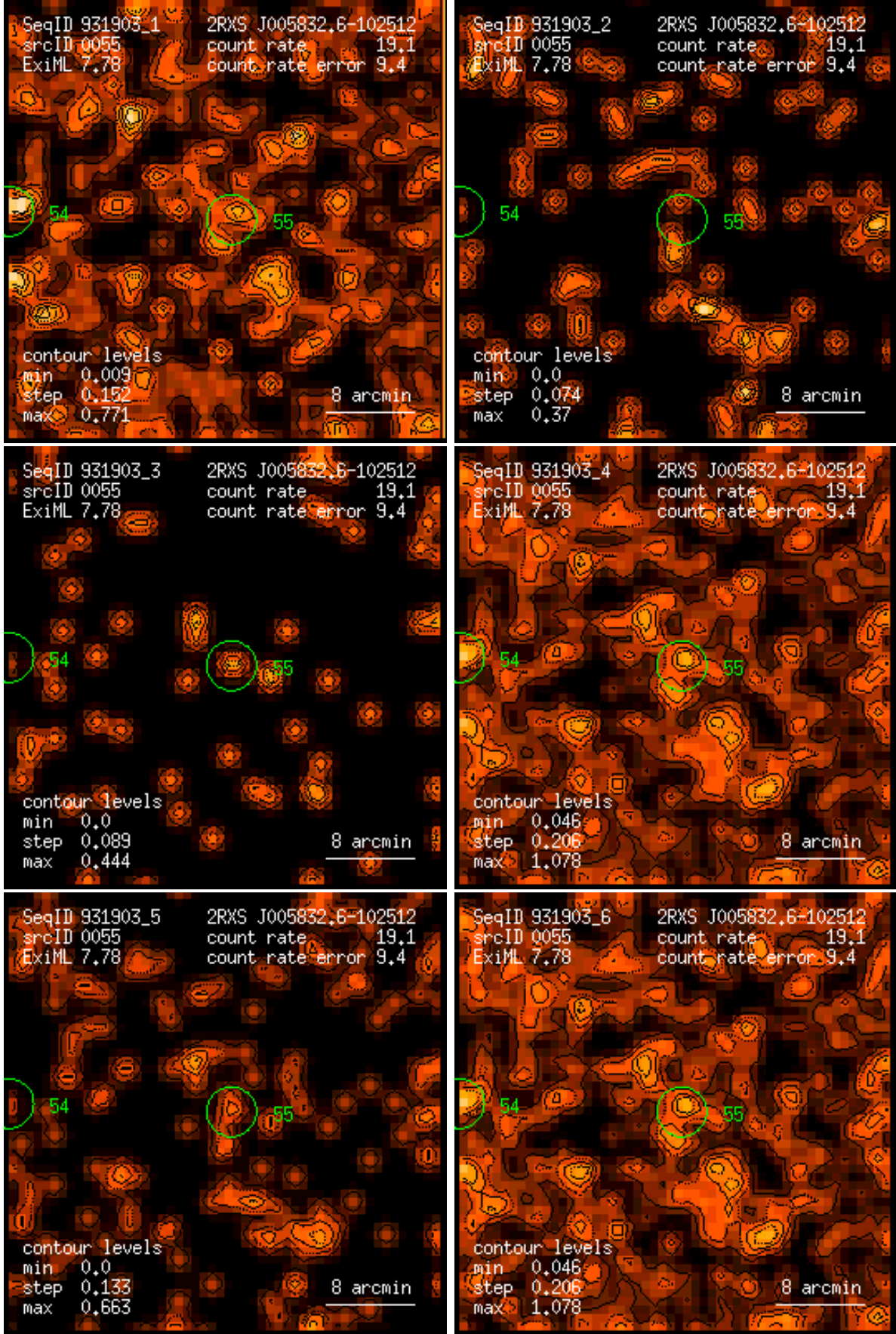
Figure 55: RASS 931903: detection 0055: band rate images, Gaussian filter: (1) PSPC channels 11 – 41, (2) 52 – 90, (3) 91 – 201, (4) 11 – 235, (5) 52 – 201, (6) 11 – 201. Broad band rates in counts/ks. Band rate contour levels in counts/ks/arcmin 2 .
