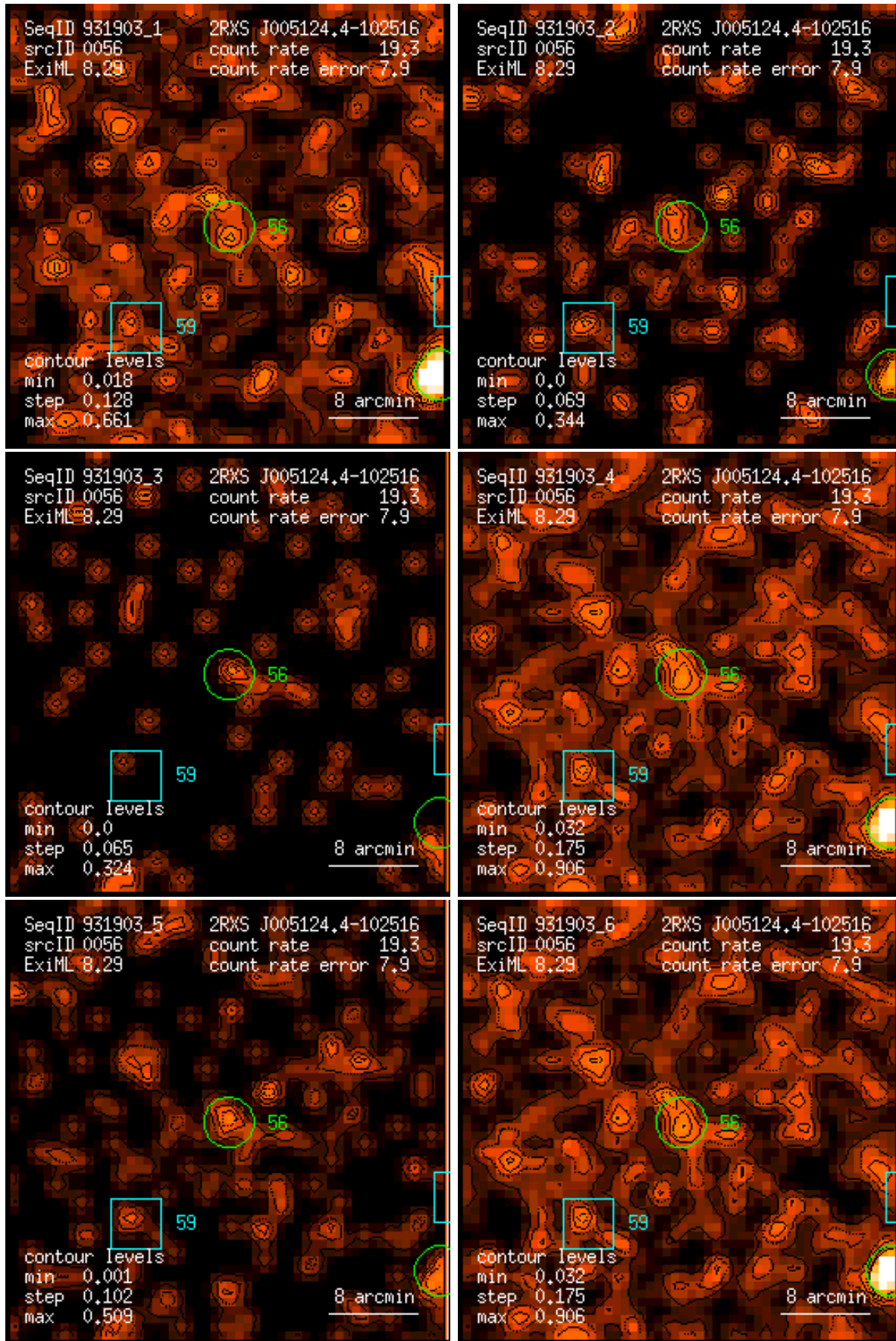
Figure 56: RASS 931903: detection 0056: band rate images, Gaussian filter: (1) PSPC channels 11 – 41, (2) 52 – 90, (3) 91 – 201, (4) 11 – 235, (5) 52 – 201, (6) 11 – 201. Broad band rates in counts/ks. Band rate contour levels in counts/ks/arcmin 2 .
