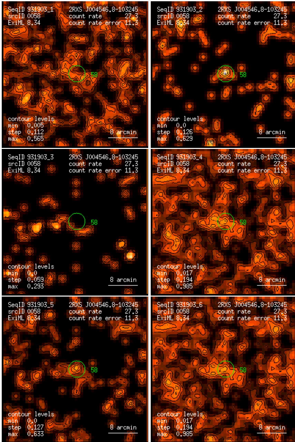
Figure 58: RASS 931903: detection 0058: band rate images, Gaussian filter: (1) PSPC channels 11 – 41, (2) 52 – 90, (3) 91 – 201, (4) 11 – 235, (5) 52 – 201, (6) 11 – 201. Broad band rates in counts/ks. Band rate contour levels in counts/ks/arcmin 2 .
