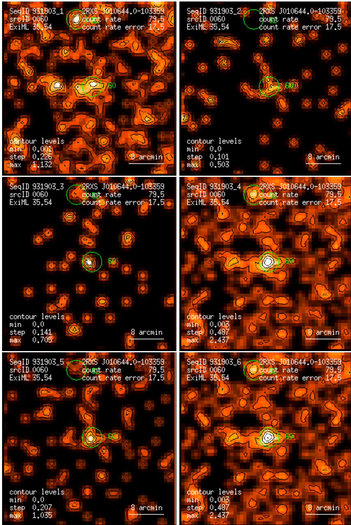
Figure 60: RASS 931903: detection 0060: band rate images, Gaussian filter: (1) PSPC channels 11 – 41, (2) 52 – 90, (3) 91 – 201, (4) 11 – 235, (5) 52 – 201, (6) 11 – 201. Broad band rates in counts/ks. Band rate contour levels in counts/ks/arcmin 2 .
