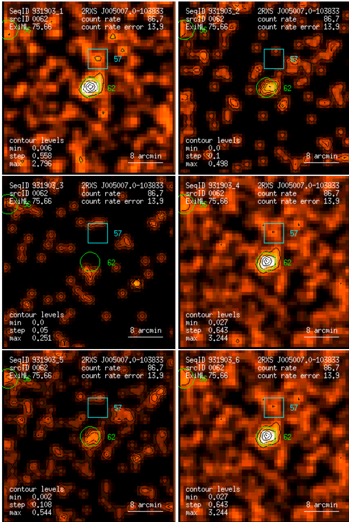
Figure 62: RASS 931903: detection 0062: band rate images, Gaussian filter: (1) PSPC channels 11 – 41, (2) 52 – 90, (3) 91 – 201, (4) 11 – 235, (5) 52 – 201, (6) 11 – 201. Broad band rates in counts/ks. Band rate contour levels in counts/ks/arcmin 2 .
