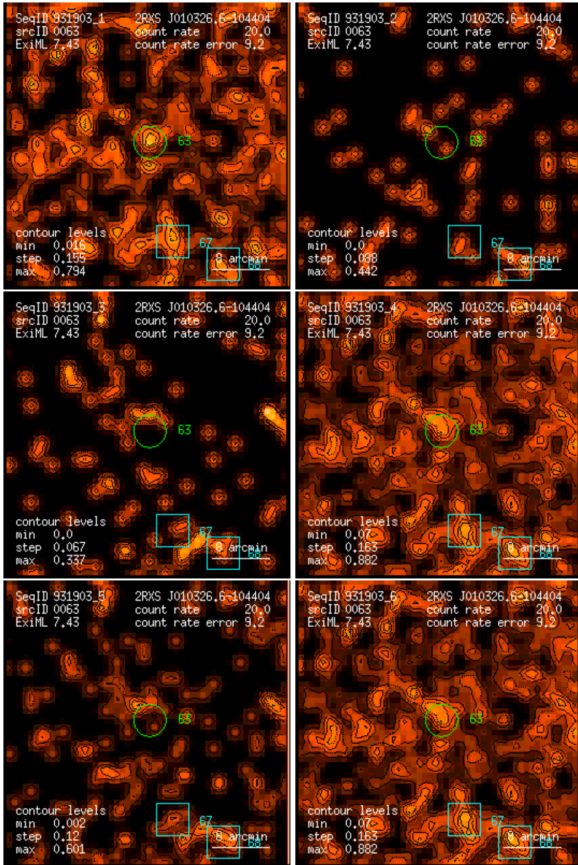
Figure 63: RASS 931903: detection 0063: band rate images, Gaussian filter: (1) PSPC channels 11 – 41, (2) 52 – 90, (3) 91 – 201, (4) 11 – 235, (5) 52 – 201, (6) 11 – 201. Broad band rates in counts/ks. Band rate contour levels in counts/ks/arcmin 2 .
