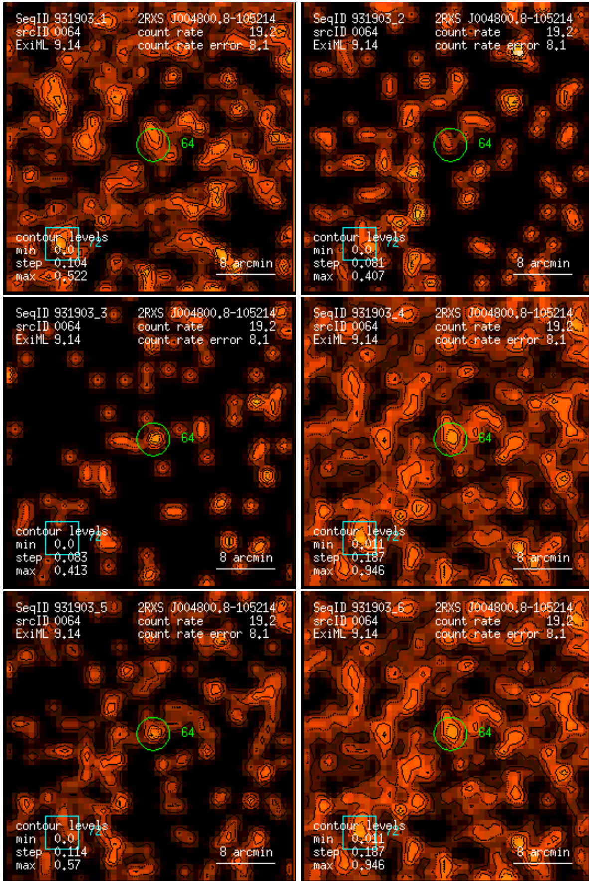
Figure 64: RASS 931903: detection 0064: band rate images, Gaussian filter: (1) PSPC channels 11 – 41, (2) 52 – 90, (3) 91 – 201, (4) 11 – 235, (5) 52 – 201, (6) 11 – 201. Broad band rates in counts/ks. Band rate contour levels in counts/ks/arcmin 2 .
