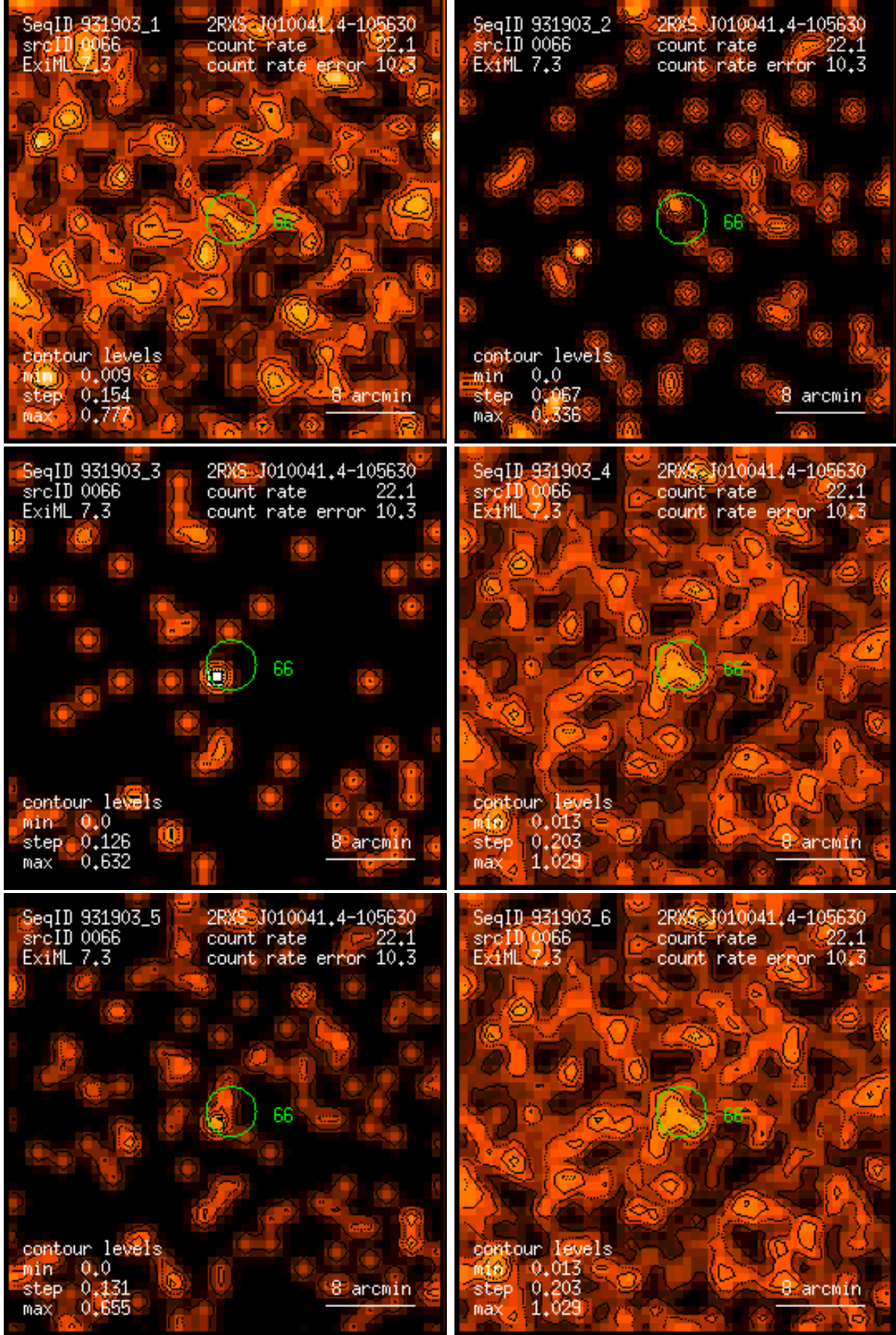
Figure 66: RASS 931903: detection 0066: band rate images, Gaussian filter: (1) PSPC channels 11 – 41, (2) 52 – 90, (3) 91 – 201, (4) 11 – 235, (5) 52 – 201, (6) 11 – 201. Broad band rates in counts/ks. Band rate contour levels in counts/ks/arcmin 2 .
