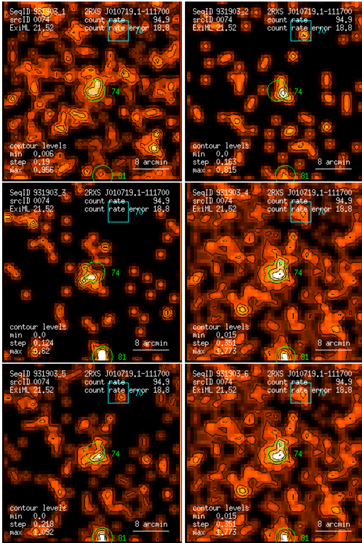
Figure 74: RASS 931903: detection 0074: band rate images, Gaussian filter: (1) PSPC channels 11 – 41, (2) 52 – 90, (3) 91 – 201, (4) 11 – 235, (5) 52 – 201, (6) 11 – 201. Broad band rates in counts/ks. Band rate contour levels in counts/ks/arcmin 2 .
