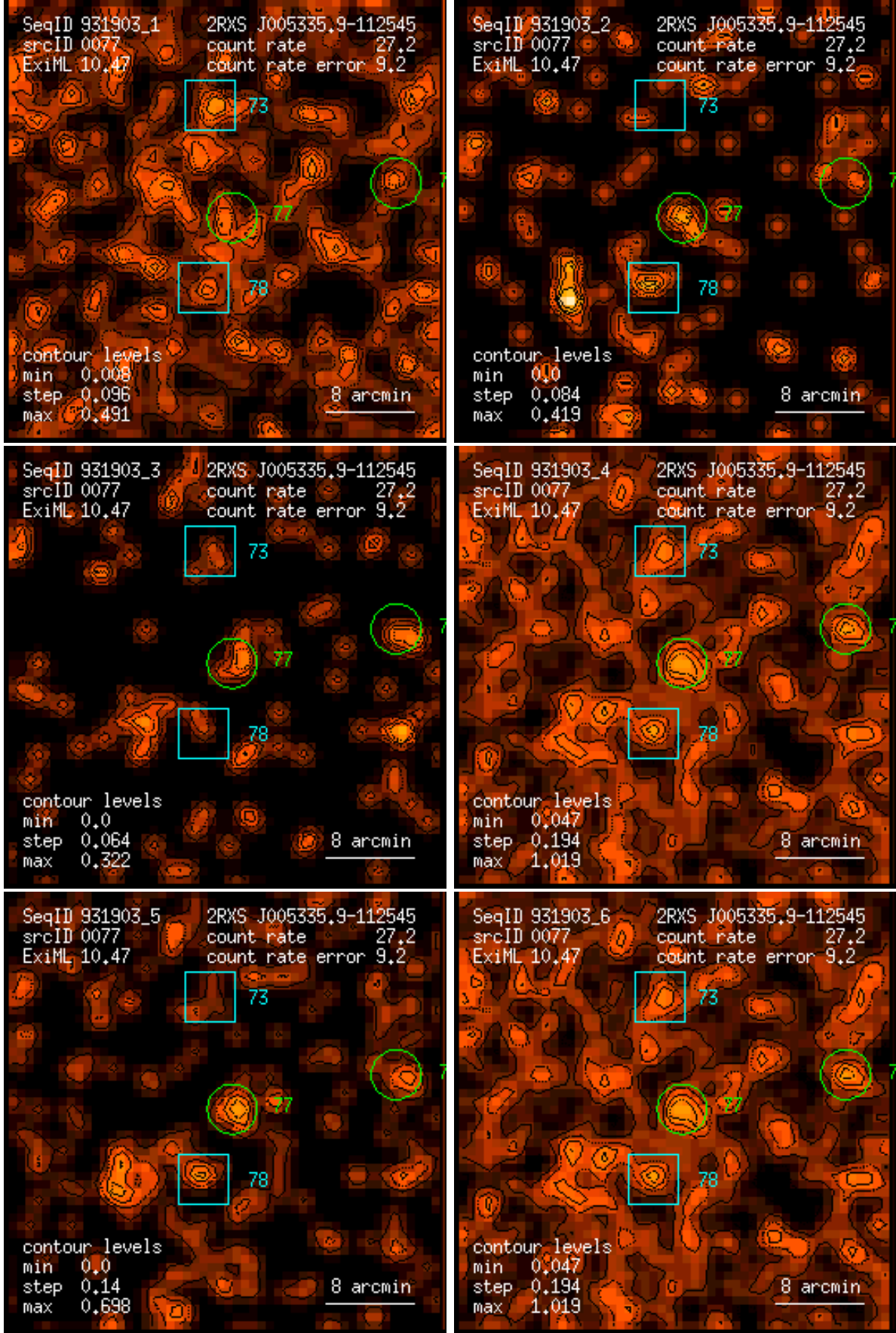
Figure 77: RASS 931903: detection 0077: band rate images, Gaussian filter: (1) PSPC channels 11 – 41, (2) 52 – 90, (3) 91 – 201, (4) 11 – 235, (5) 52 – 201, (6) 11 – 201. Broad band rates in counts/ks. Band rate contour levels in counts/ks/arcmin 2 .
