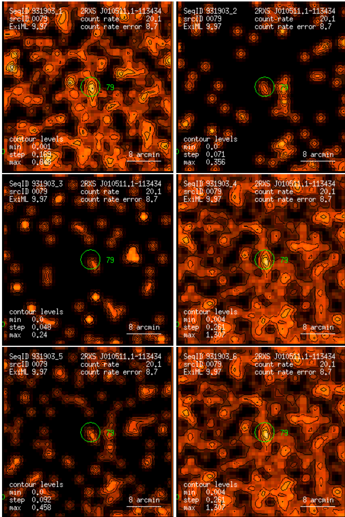
Figure 79: RASS 931903: detection 0079: band rate images, Gaussian filter: (1) PSPC channels 11 – 41, (2) 52 – 90, (3) 91 – 201, (4) 11 – 235, (5) 52 – 201, (6) 11 – 201. Broad band rates in counts/ks. Band rate contour levels in counts/ks/arcmin 2 .
