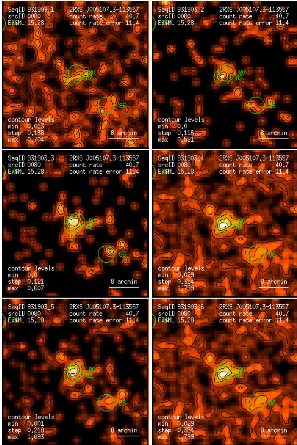
Figure 80: RASS 931903: detection 0080: band rate images, Gaussian filter: (1) PSPC channels 11 – 41, (2) 52 – 90, (3) 91 – 201, (4) 11 – 235, (5) 52 – 201, (6) 11 – 201. Broad band rates in counts/ks. Band rate contour levels in counts/ks/arcmin 2 .
