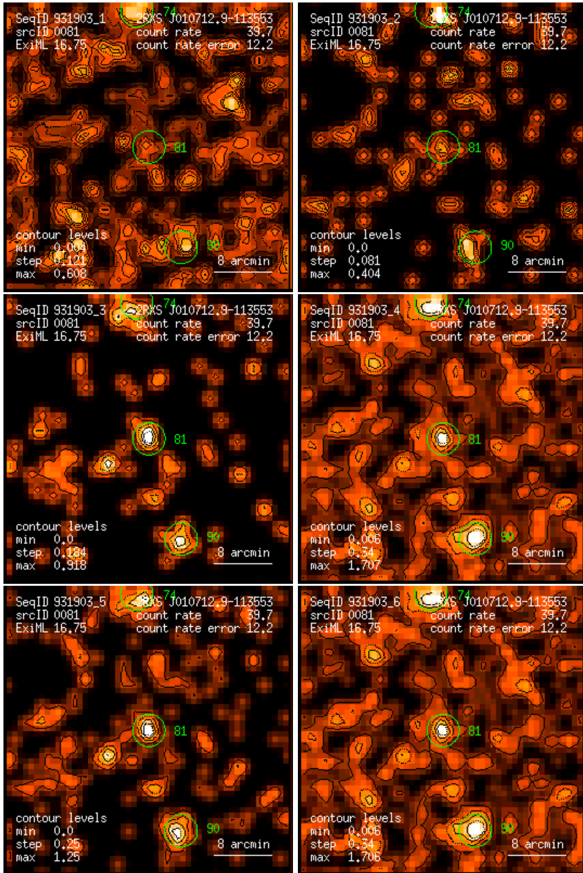
Figure 81: RASS 931903: detection 0081: band rate images, Gaussian filter: (1) PSPC channels 11 – 41, (2) 52 – 90, (3) 91 – 201, (4) 11 – 235, (5) 52 – 201, (6) 11 – 201. Broad band rates in counts/ks. Band rate contour levels in counts/ks/arcmin 2 .
