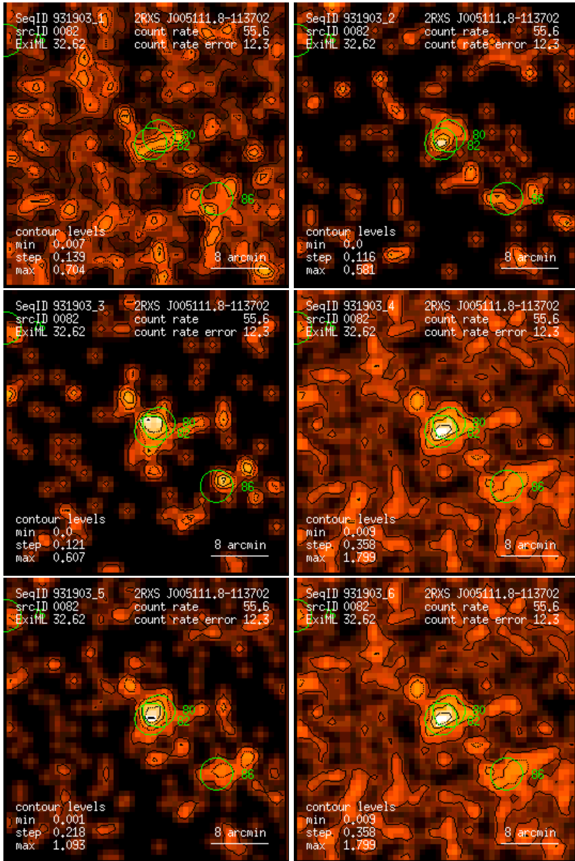
Figure 82: RASS 931903: detection 0082: band rate images, Gaussian filter: (1) PSPC channels 11 – 41, (2) 52 – 90, (3) 91 – 201, (4) 11 – 235, (5) 52 – 201, (6) 11 – 201. Broad band rates in counts/ks. Band rate contour levels in counts/ks/arcmin 2 .
