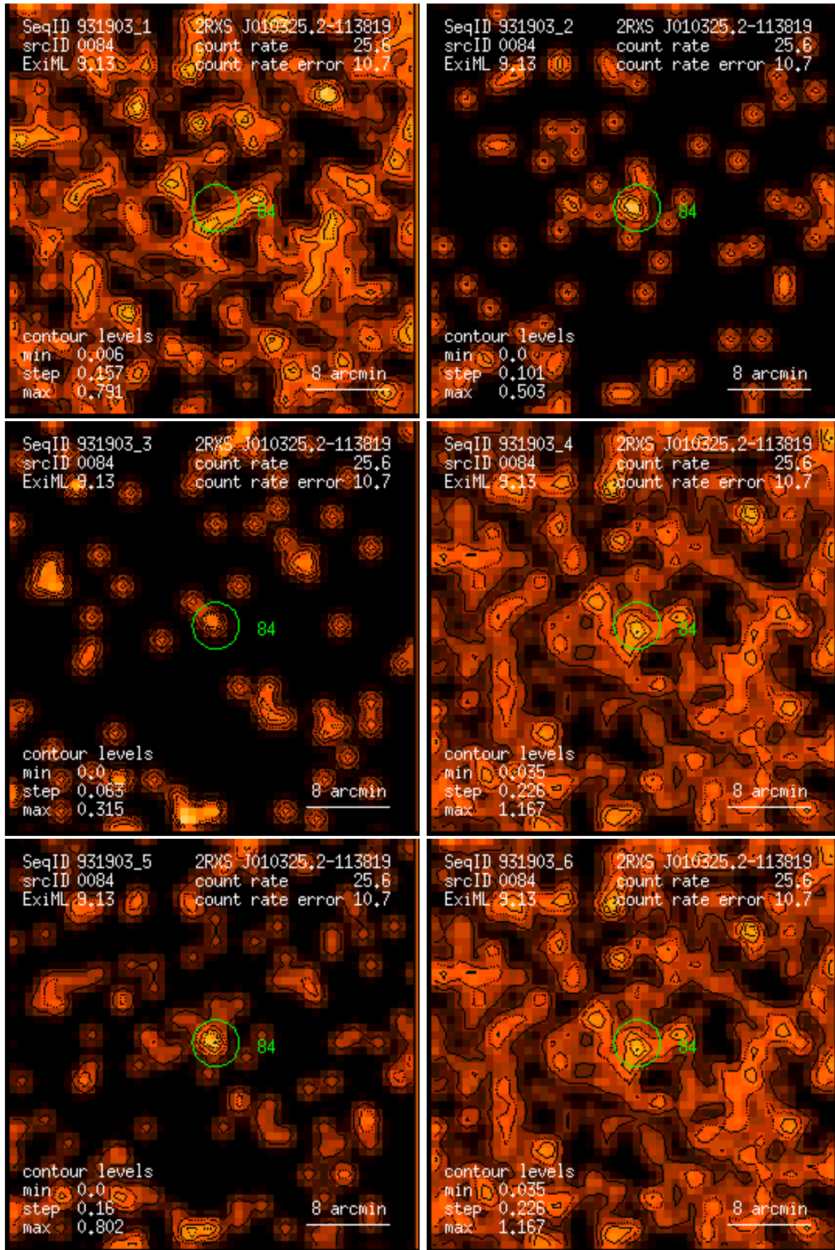
Figure 84: RASS 931903: detection 0084: band rate images, Gaussian filter: (1) PSPC channels 11 – 41, (2) 52 – 90, (3) 91 – 201, (4) 11 – 235, (5) 52 – 201, (6) 11 – 201. Broad band rates in counts/ks. Band rate contour levels in counts/ks/arcmin 2 .
