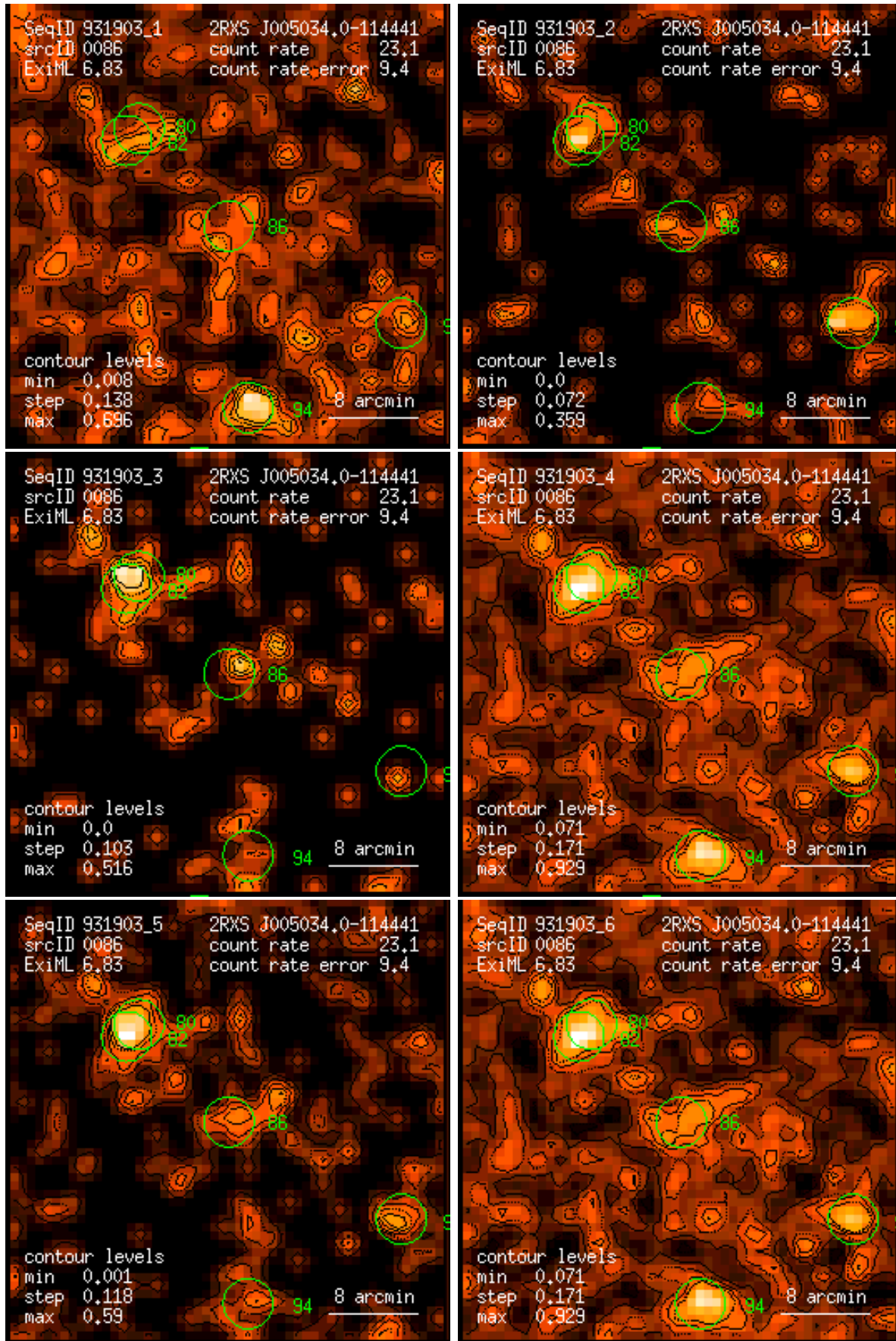
Figure 86: RASS 931903: detection 0086: band rate images, Gaussian filter: (1) PSPC channels 11 – 41, (2) 52 – 90, (3) 91 – 201, (4) 11 – 235, (5) 52 – 201, (6) 11 – 201. Broad band rates in counts/ks. Band rate contour levels in counts/ks/arcmin 2 .
