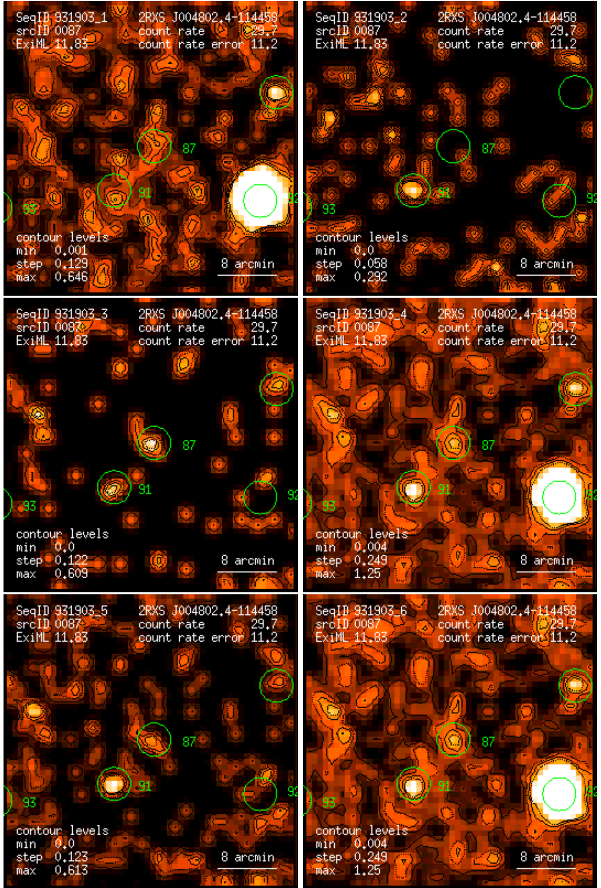
Figure 87: RASS 931903: detection 0087: band rate images, Gaussian filter: (1) PSPC channels 11 – 41, (2) 52 – 90, (3) 91 – 201, (4) 11 – 235, (5) 52 – 201, (6) 11 – 201. Broad band rates in counts/ks. Band rate contour levels in counts/ks/arcmin 2 .
