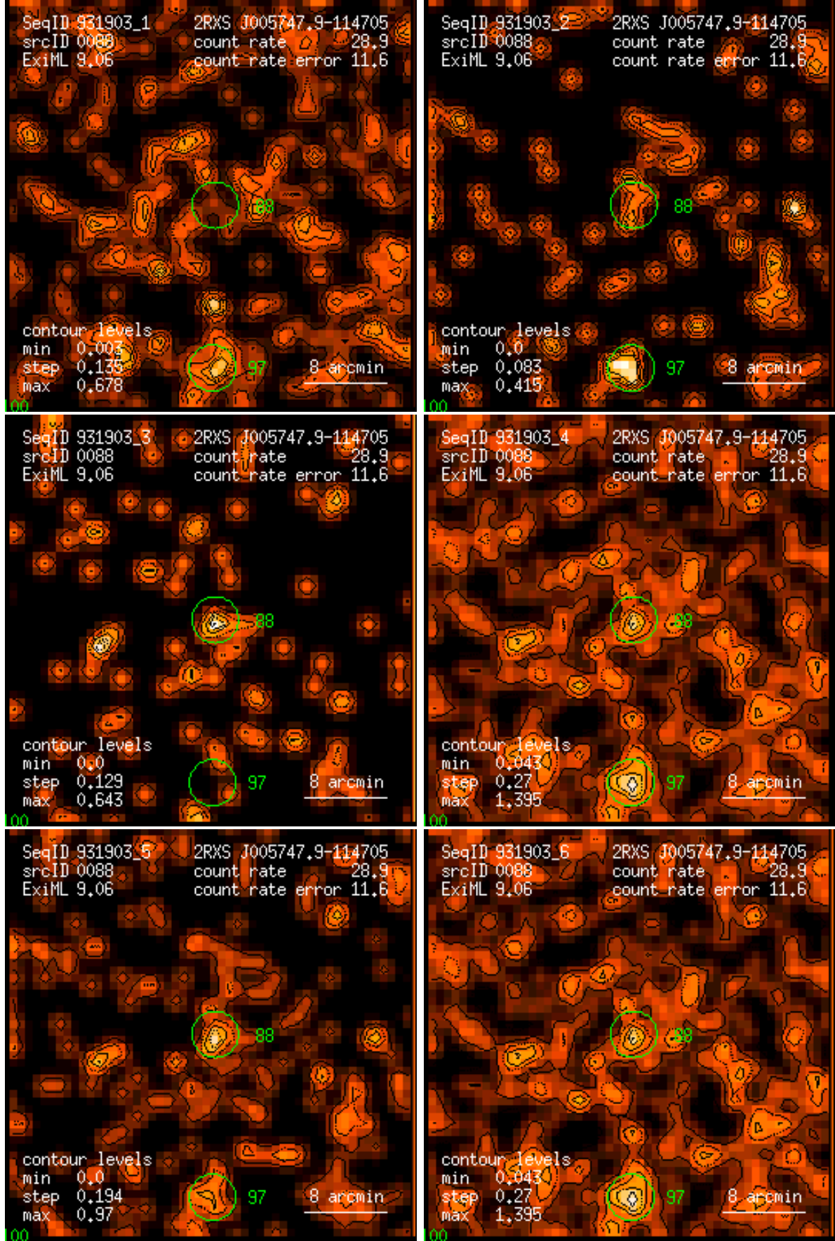
Figure 88: RASS 931903: detection 0088: band rate images, Gaussian filter: (1) PSPC channels 11 – 41, (2) 52 – 90, (3) 91 – 201, (4) 11 – 235, (5) 52 – 201, (6) 11 – 201. Broad band rates in counts/ks. Band rate contour levels in counts/ks/arcmin 2 .
