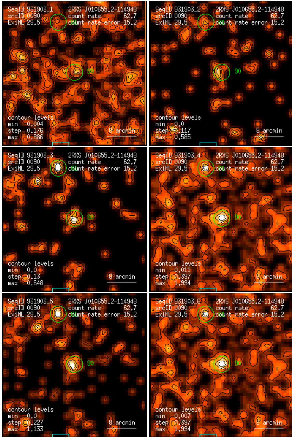
Figure 90: RASS 931903: detection 0090: band rate images, Gaussian filter: (1) PSPC channels 11 – 41, (2) 52 – 90, (3) 91 – 201, (4) 11 – 235, (5) 52 – 201, (6) 11 – 201. Broad band rates in counts/ks. Band rate contour levels in counts/ks/arcmin 2 .
