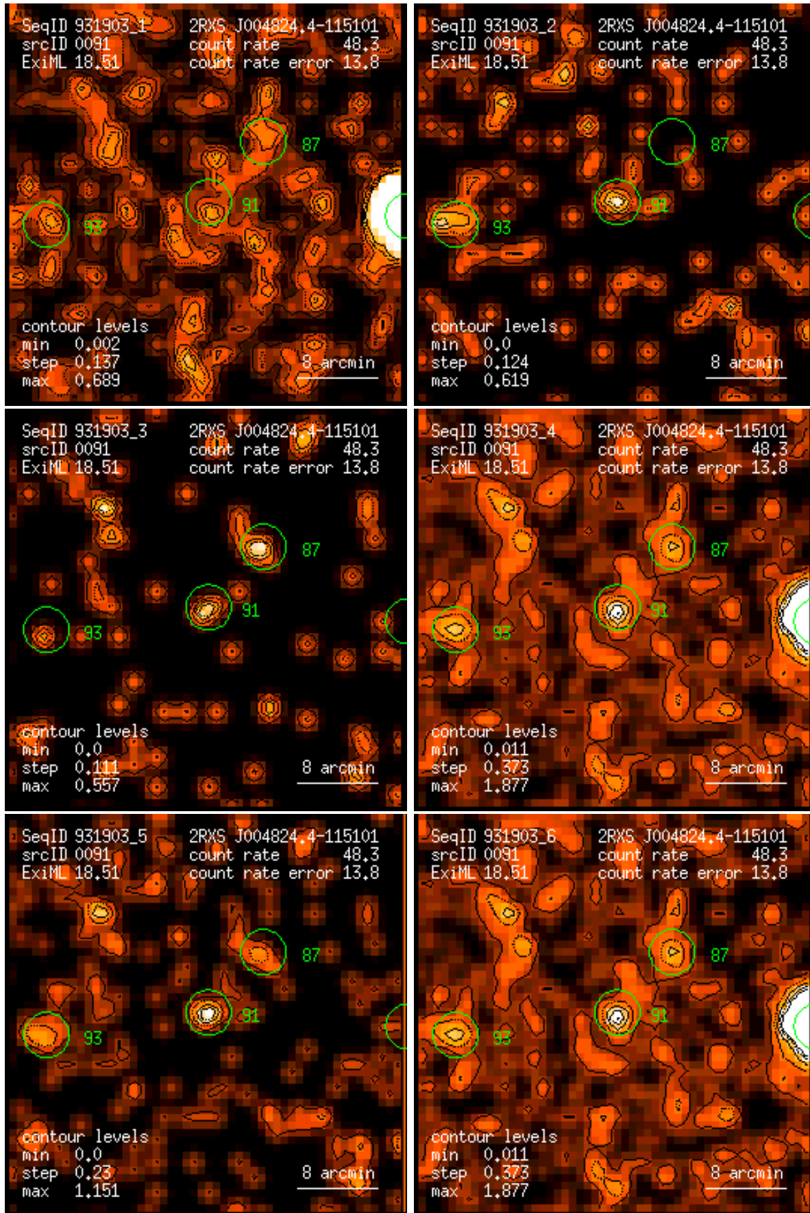
Figure 91: RASS 931903: detection 0091: band rate images, Gaussian filter: (1) PSPC channels 11 – 41, (2) 52 – 90, (3) 91 – 201, (4) 11 – 235, (5) 52 – 201, (6) 11 – 201. Broad band rates in counts/ks. Band rate contour levels in counts/ks/arcmin 2 .
