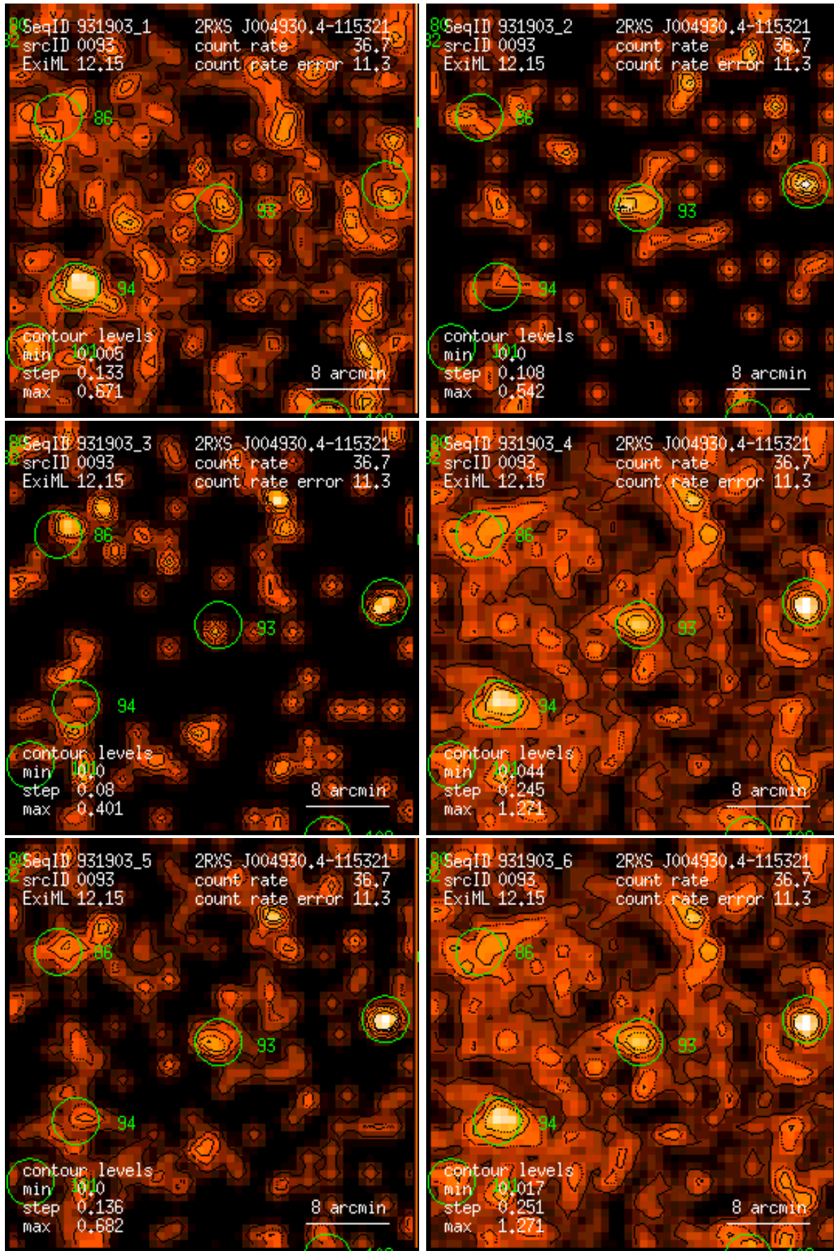
Figure 93: RASS 931903: detection 0093: band rate images, Gaussian filter: (1) PSPC channels 11 – 41, (2) 52 – 90, (3) 91 – 201, (4) 11 – 235, (5) 52 – 201, (6) 11 – 201. Broad band rates in counts/ks. Band rate contour levels in counts/ks/arcmin 2 .
