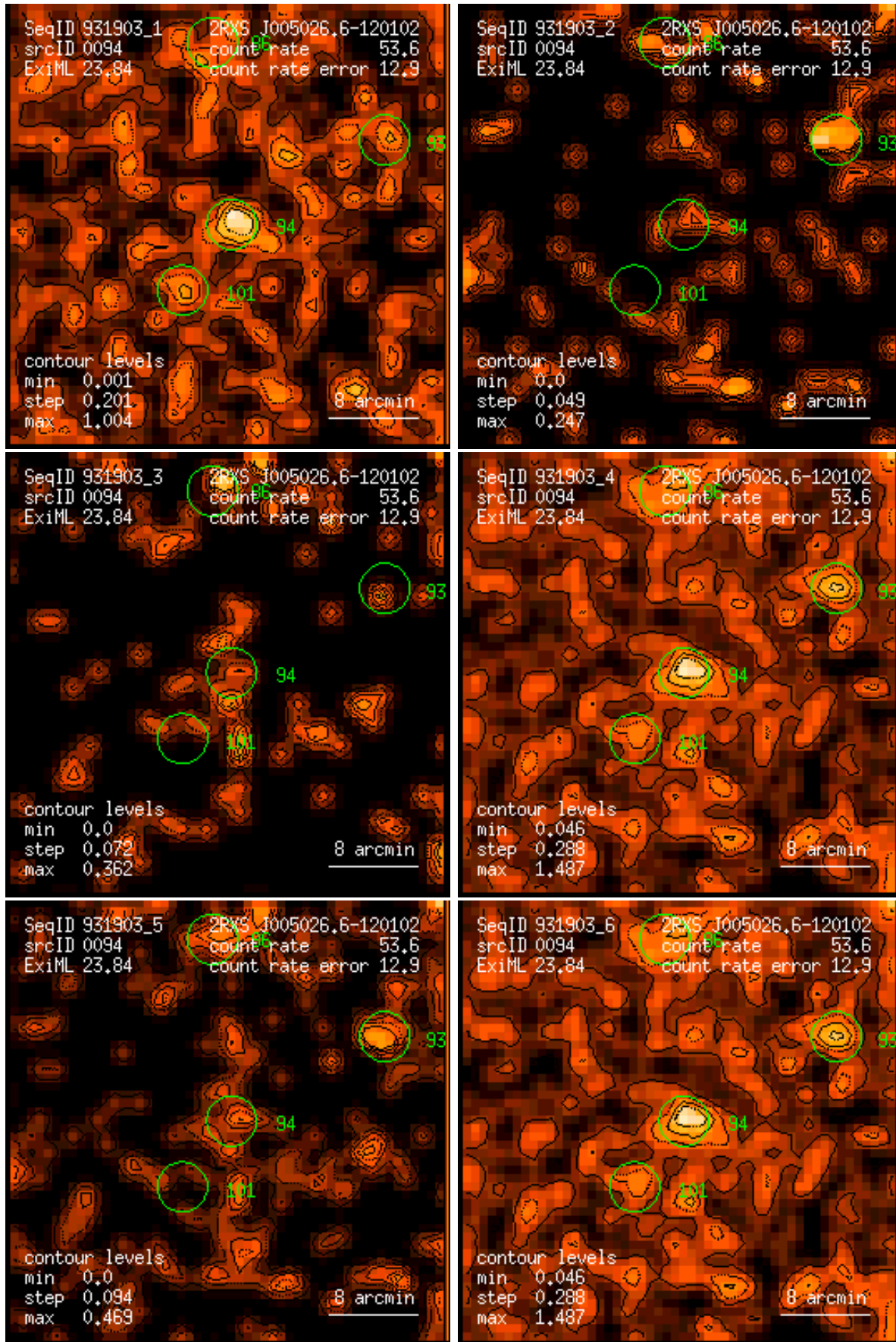
Figure 94: RASS 931903: detection 0094: band rate images, Gaussian filter: (1) PSPC channels 11 – 41, (2) 52 – 90, (3) 91 – 201, (4) 11 – 235, (5) 52 – 201, (6) 11 – 201. Broad band rates in counts/ks. Band rate contour levels in counts/ks/arcmin 2 .
