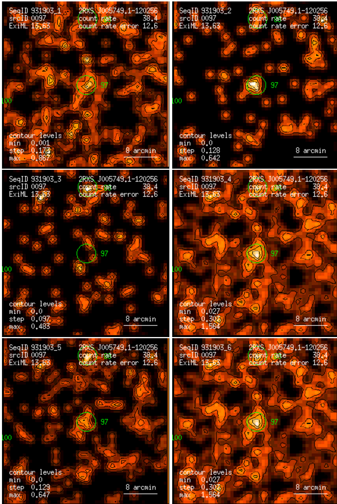
Figure 97: RASS 931903: detection 0097: band rate images, Gaussian filter: (1) PSPC channels 11 – 41, (2) 52 – 90, (3) 91 – 201, (4) 11 – 235, (5) 52 – 201, (6) 11 – 201. Broad band rates in counts/ks. Band rate contour levels in counts/ks/arcmin 2 .
