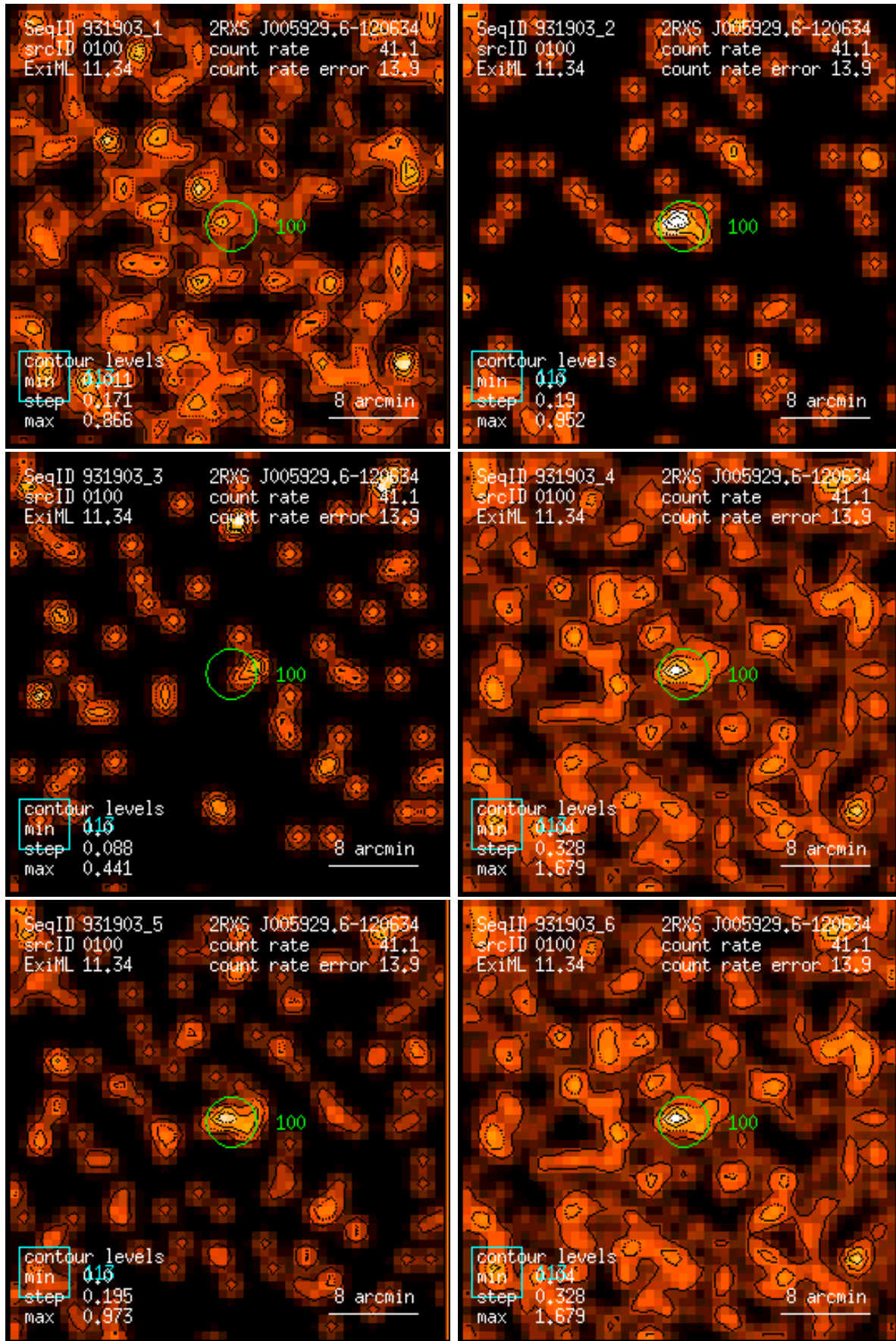
Figure 100: RASS 931903: detection 0100: band rate images, Gaussian filter: (1) PSPC channels 11 – 41, (2) 52 – 90, (3) 91 – 201, (4) 11 – 235, (5) 52 – 201, (6) 11 – 201. Broad band rates in counts/ks. Band rate contour levels in counts/ks/arcmin 2 .
