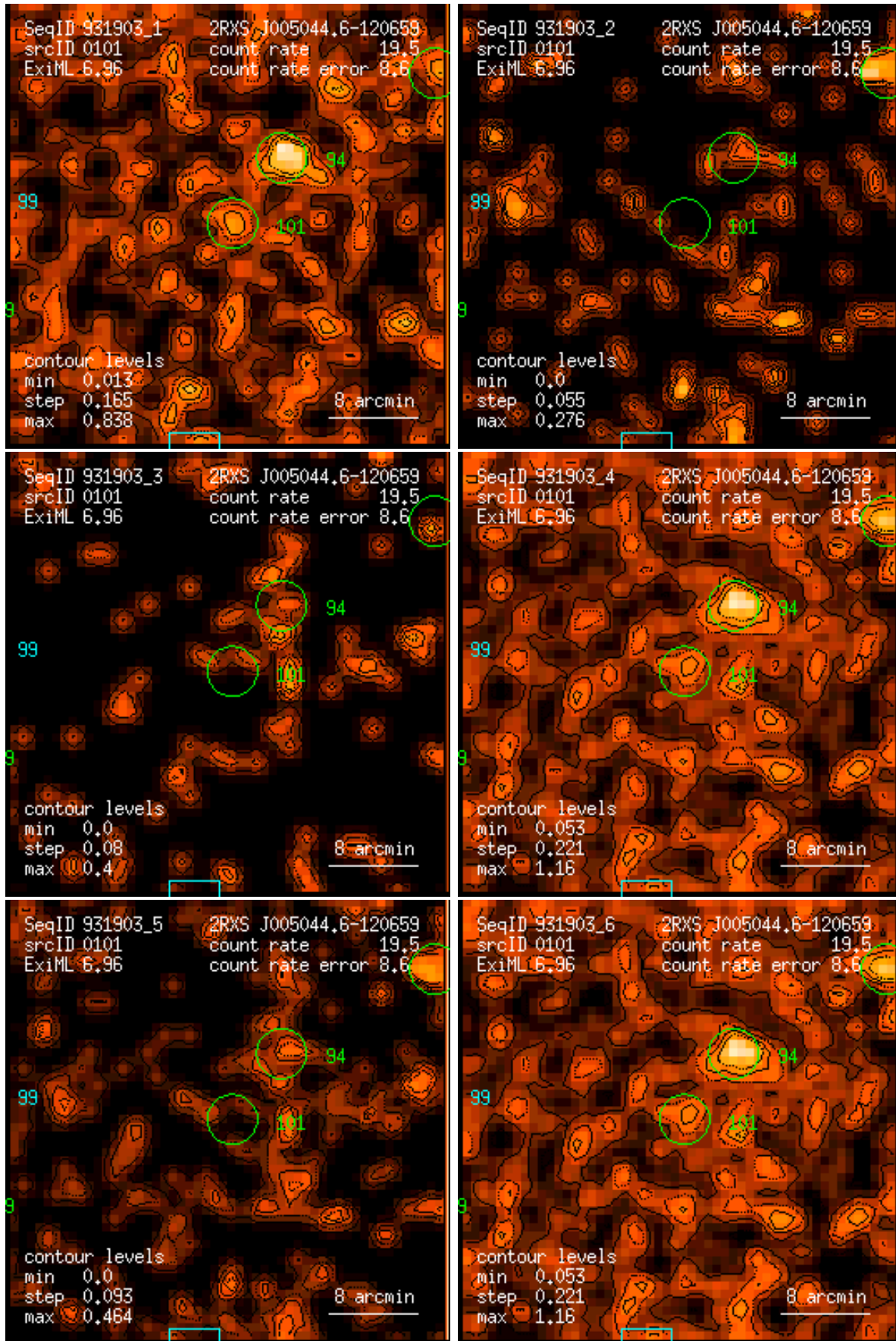
Figure 101: RASS 931903: detection 0101: band rate images, Gaussian filter: (1) PSPC channels 11 – 41, (2) 52 – 90, (3) 91 – 201, (4) 11 – 235, (5) 52 – 201, (6) 11 – 201. Broad band rates in counts/ks. Band rate contour levels in counts/ks/arcmin 2 .
