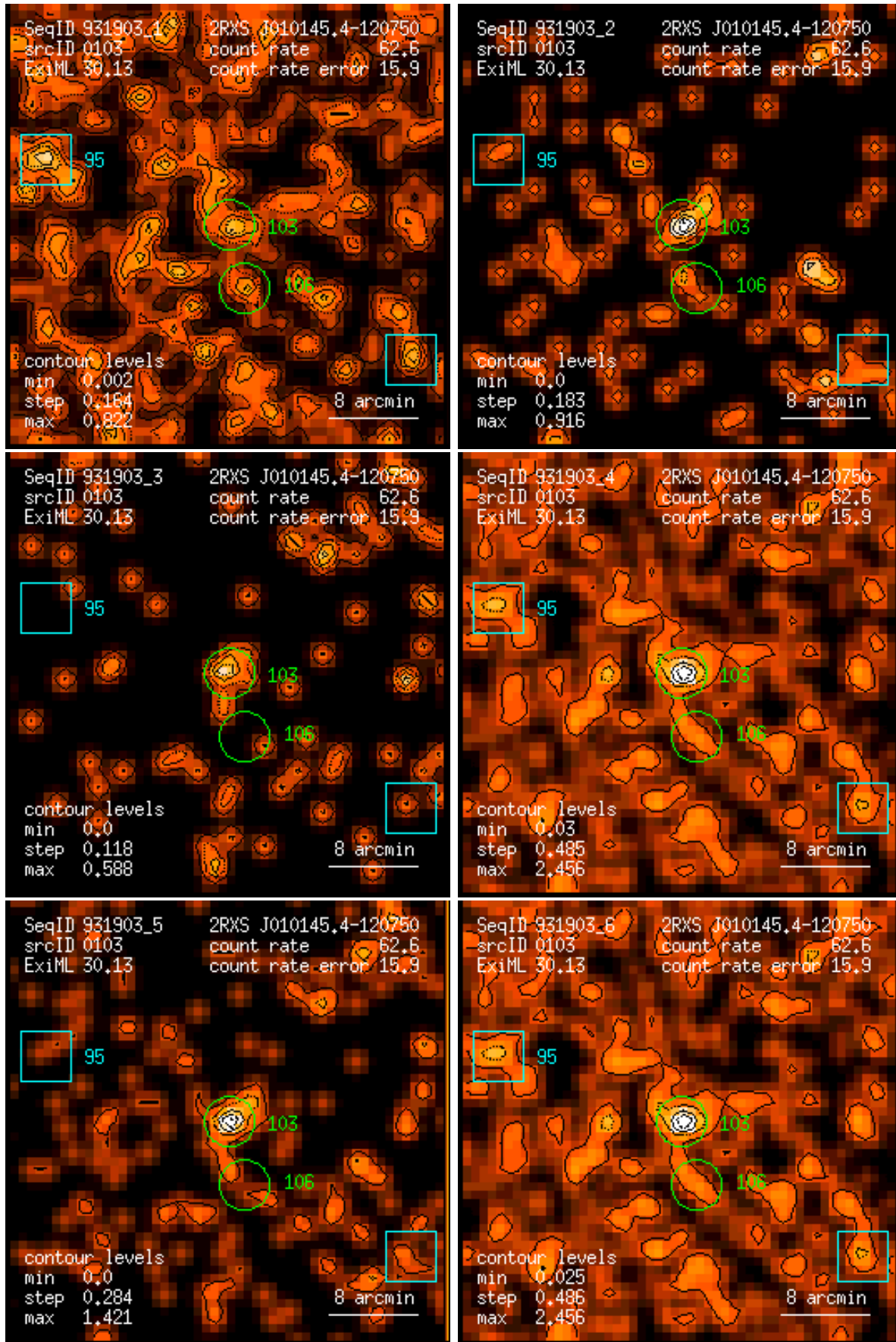
Figure 103: RASS 931903: detection 0103: band rate images, Gaussian filter: (1) PSPC channels 11 – 41, (2) 52 – 90, (3) 91 – 201, (4) 11 – 235, (5) 52 – 201, (6) 11 – 201. Broad band rates in counts/ks. Band rate contour levels in counts/ks/arcmin 2 .
