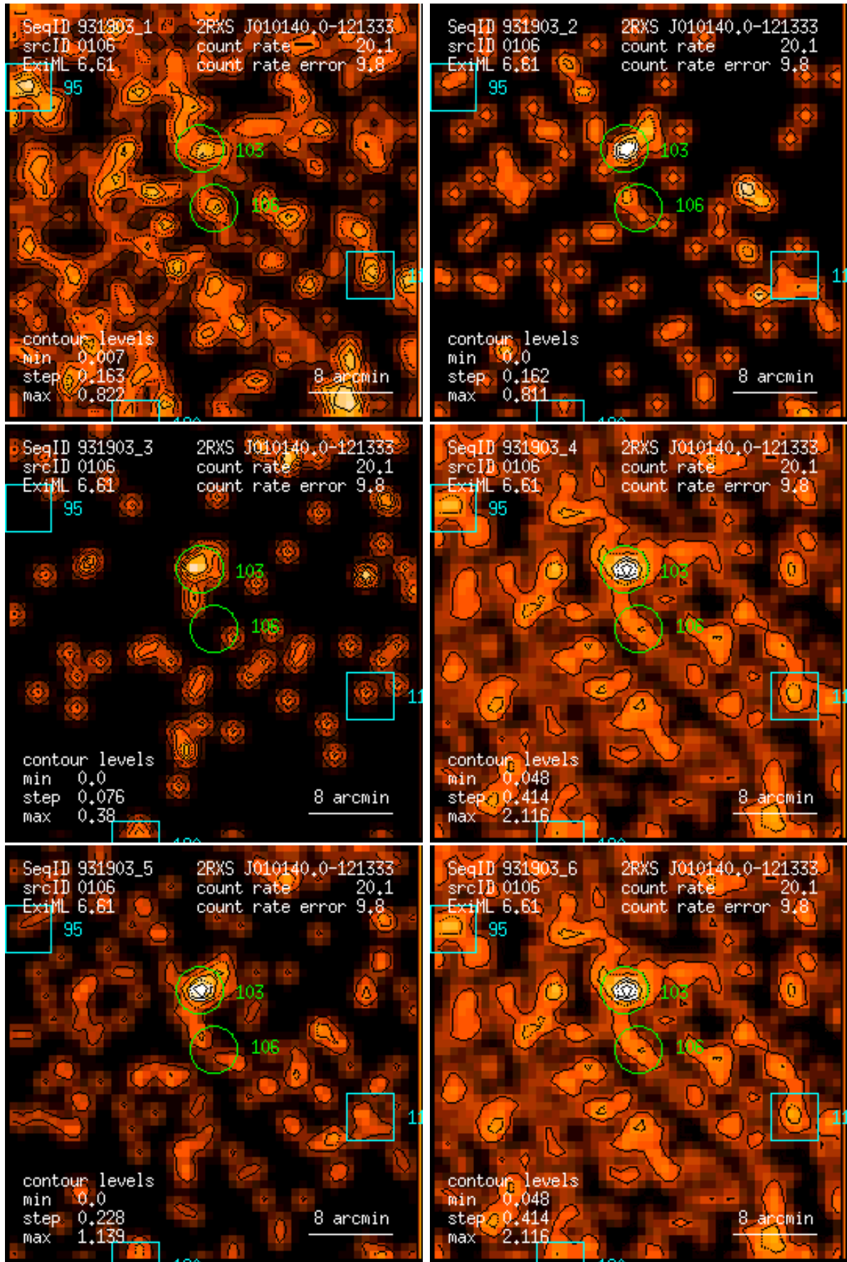
Figure 106: RASS 931903: detection 0106: band rate images, Gaussian filter: (1) PSPC channels 11 – 41, (2) 52 – 90, (3) 91 – 201, (4) 11 – 235, (5) 52 – 201, (6) 11 – 201. Broad band rates in counts/ks. Band rate contour levels in counts/ks/arcmin 2 .
