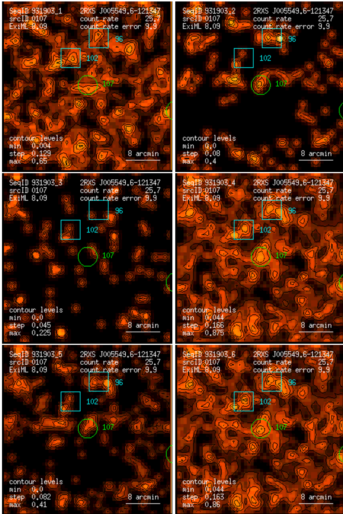
Figure 107: RASS 931903: detection 0107: band rate images, Gaussian filter: (1) PSPC channels 11 – 41, (2) 52 – 90, (3) 91 – 201, (4) 11 – 235, (5) 52 – 201, (6) 11 – 201. Broad band rates in counts/ks. Band rate contour levels in counts/ks/arcmin 2 .
