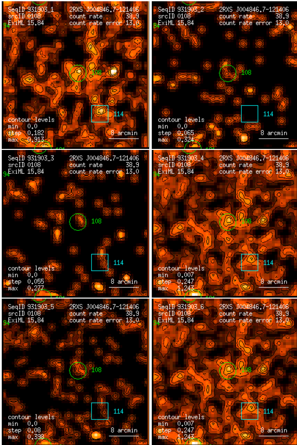
Figure 108: RASS 931903: detection 0108: band rate images, Gaussian filter: (1) PSPC channels 11 – 41, (2) 52 – 90, (3) 91 – 201, (4) 11 – 235, (5) 52 – 201, (6) 11 – 201. Broad band rates in counts/ks. Band rate contour levels in counts/ks/arcmin 2 .
