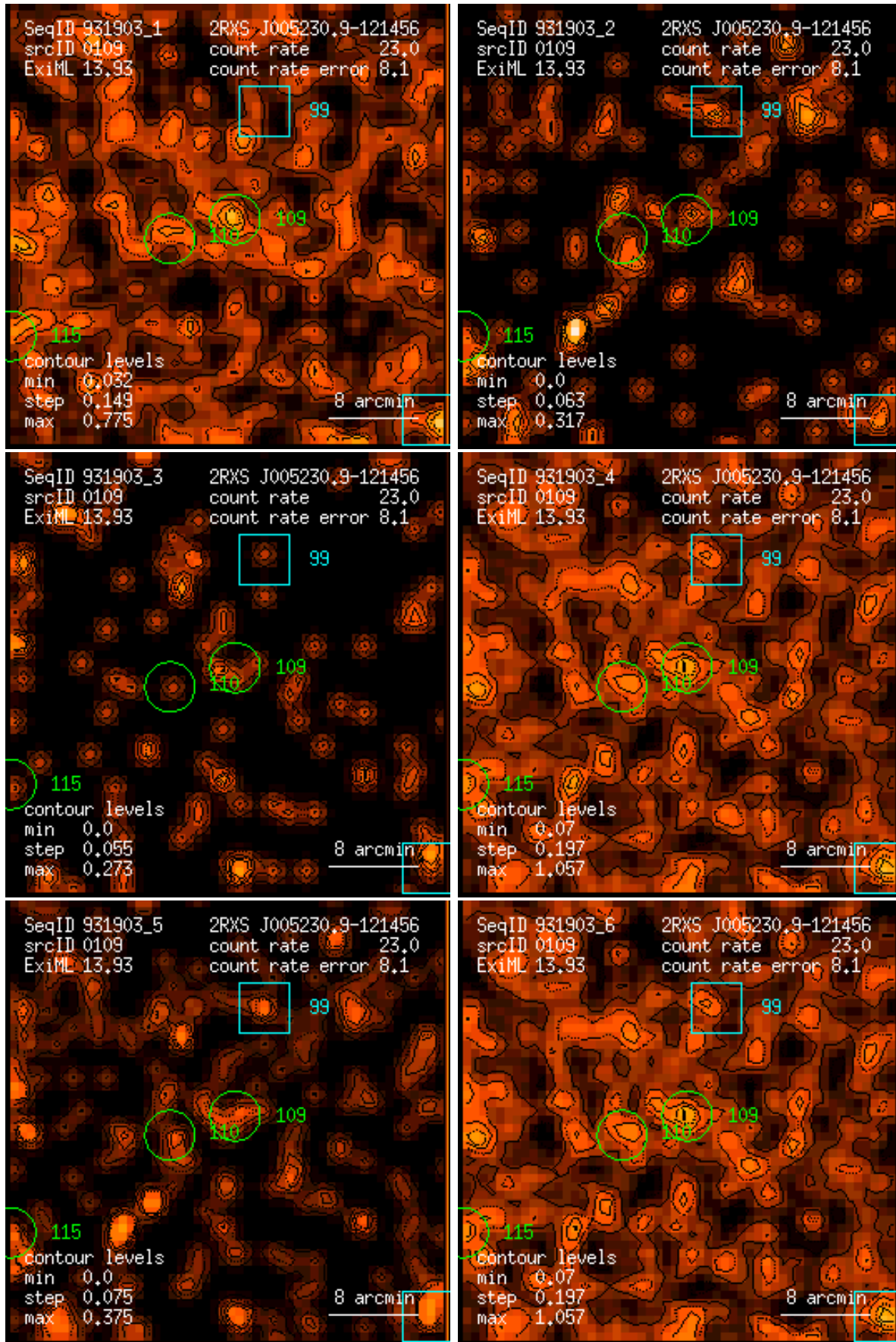
Figure 109: RASS 931903: detection 0109: band rate images, Gaussian filter: (1) PSPC channels 11 – 41, (2) 52 – 90, (3) 91 – 201, (4) 11 – 235, (5) 52 – 201, (6) 11 – 201. Broad band rates in counts/ks. Band rate contour levels in counts/ks/arcmin 2 .
