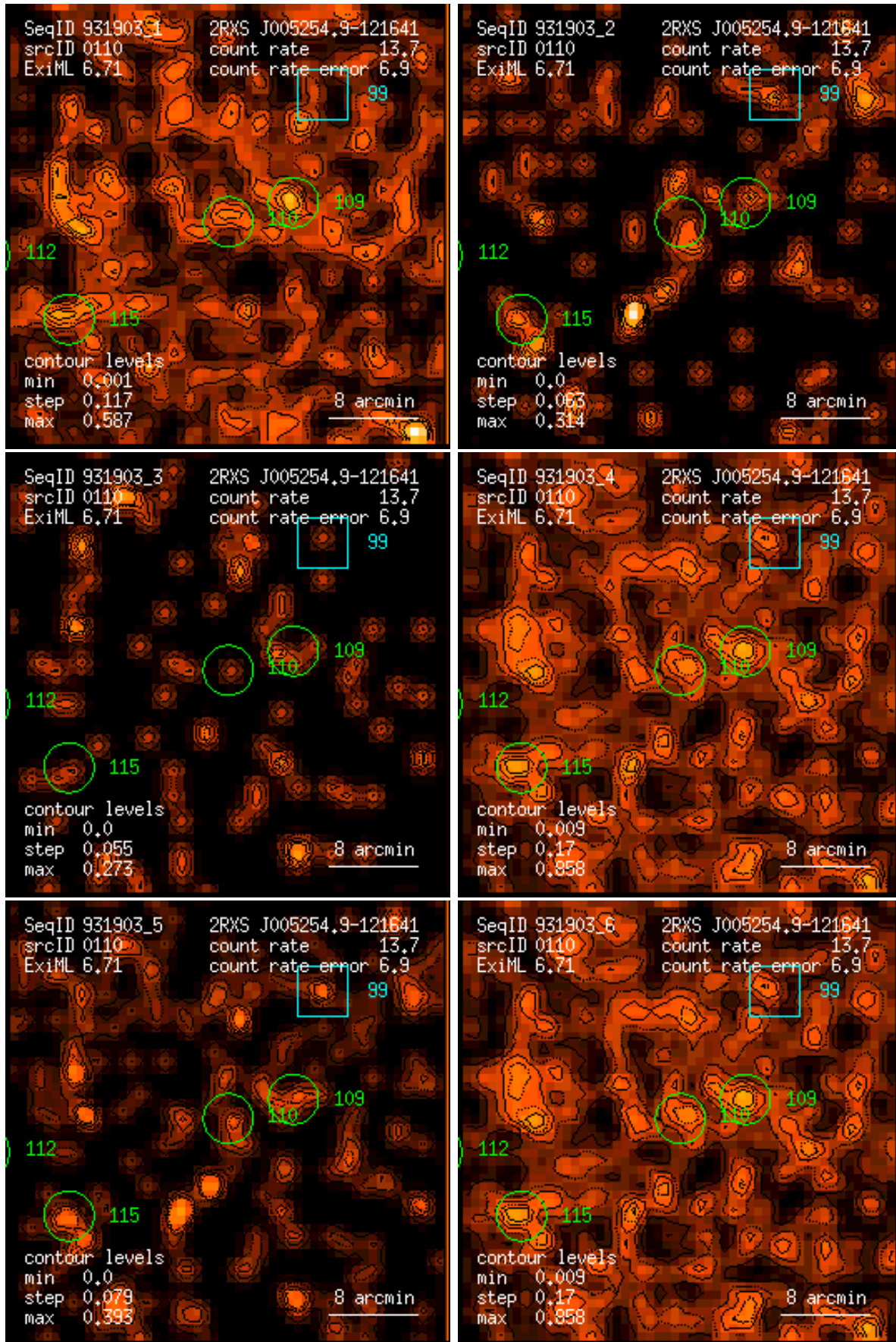
Figure 110: RASS 931903: detection 0110: band rate images, Gaussian filter: (1) PSPC channels 11 – 41, (2) 52 – 90, (3) 91 – 201, (4) 11 – 235, (5) 52 – 201, (6) 11 – 201. Broad band rates in counts/ks. Band rate contour levels in counts/ks/arcmin 2 .
