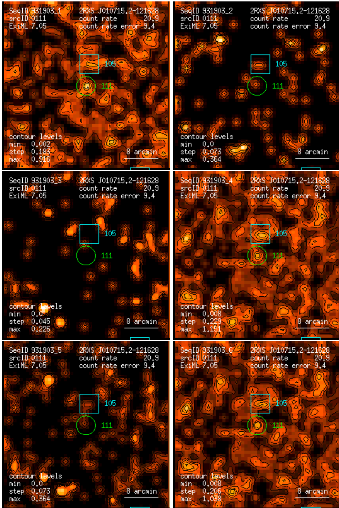
Figure 111: RASS 931903: detection 0111: band rate images, Gaussian filter: (1) PSPC channels 11 – 41, (2) 52 – 90, (3) 91 – 201, (4) 11 – 235, (5) 52 – 201, (6) 11 – 201. Broad band rates in counts/ks. Band rate contour levels in counts/ks/arcmin 2 .
