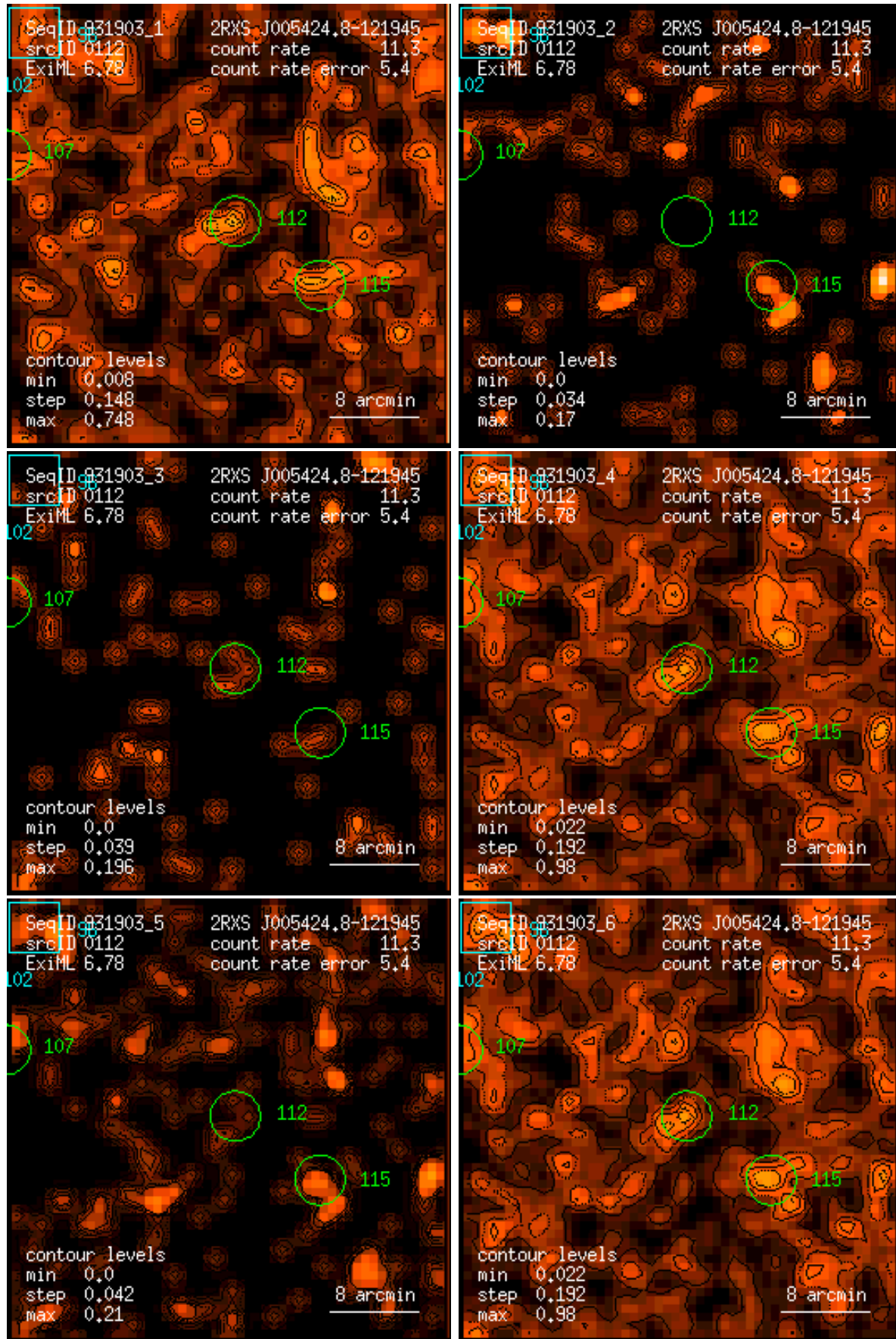
Figure 112: RASS 931903: detection 0112: band rate images, Gaussian filter: (1) PSPC channels 11 – 41, (2) 52 – 90, (3) 91 – 201, (4) 11 – 235, (5) 52 – 201, (6) 11 – 201. Broad band rates in counts/ks. Band rate contour levels in counts/ks/arcmin 2 .
