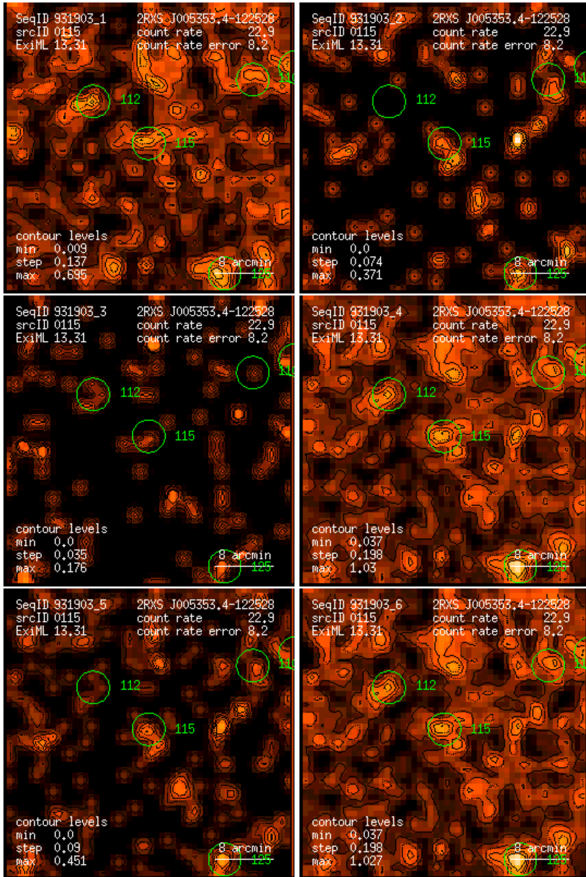
Figure 115: RASS 931903: detection 0115: band rate images, Gaussian filter: (1) PSPC channels 11 – 41, (2) 52 – 90, (3) 91 – 201, (4) 11 – 235, (5) 52 – 201, (6) 11 – 201. Broad band rates in counts/ks. Band rate contour levels in counts/ks/arcmin 2 .
