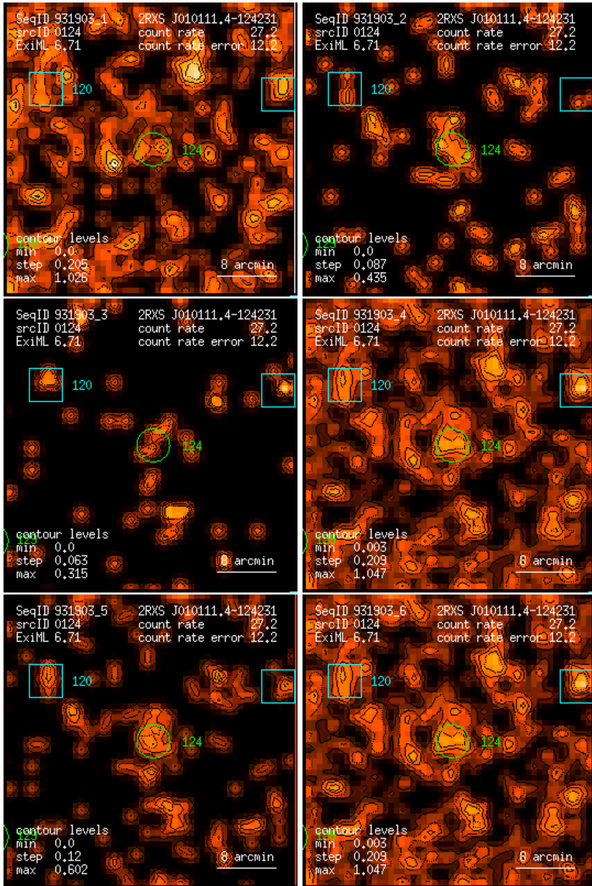
Figure 124: RASS 931903: detection 0124: band rate images, Gaussian filter: (1) PSPC channels 11 – 41, (2) 52 – 90, (3) 91 – 201, (4) 11 – 235, (5) 52 – 201, (6) 11 – 201. Broad band rates in counts/ks. Band rate contour levels in counts/ks/arcmin 2 .
