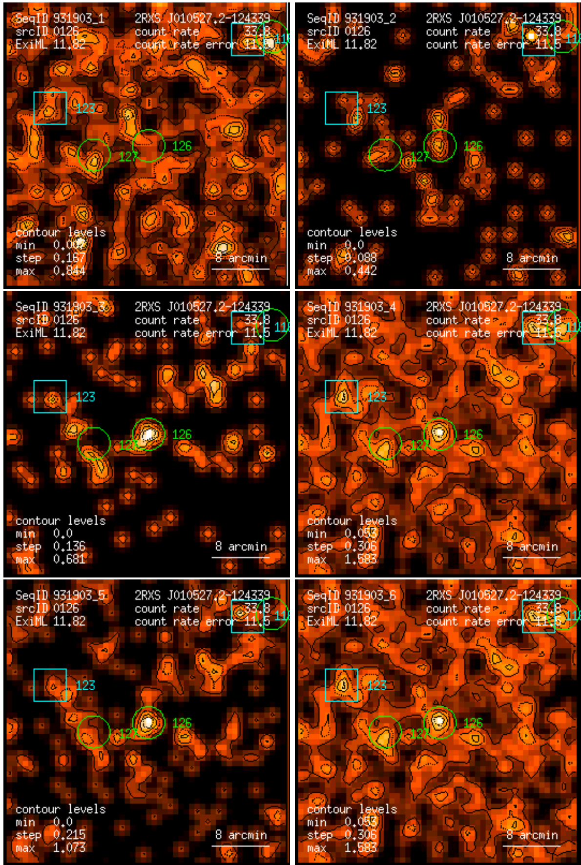
Figure 126: RASS 931903: detection 0126: band rate images, Gaussian filter: (1) PSPC channels 11 – 41, (2) 52 – 90, (3) 91 – 201, (4) 11 – 235, (5) 52 – 201, (6) 11 – 201. Broad band rates in counts/ks. Band rate contour levels in counts/ks/arcmin 2 .
