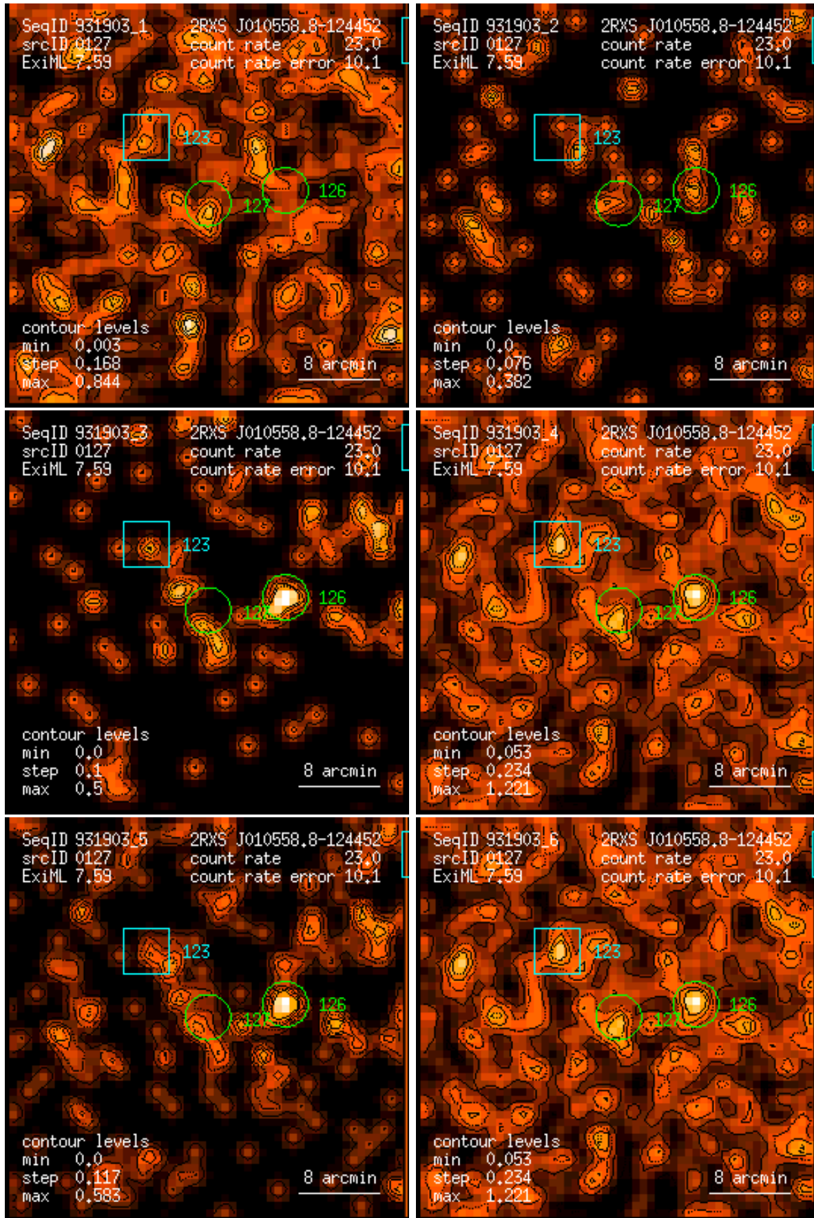
Figure 127: RASS 931903: detection 0127: band rate images, Gaussian filter: (1) PSPC channels 11 – 41, (2) 52 – 90, (3) 91 – 201, (4) 11 – 235, (5) 52 – 201, (6) 11 – 201. Broad band rates in counts/ks. Band rate contour levels in counts/ks/arcmin 2 .
