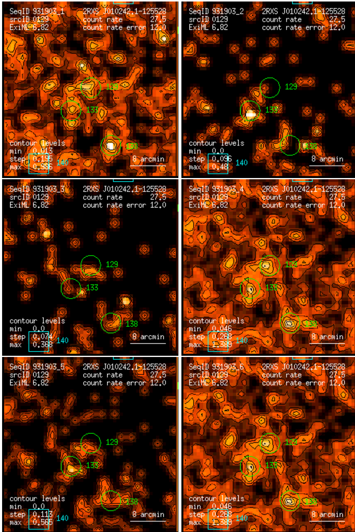
Figure 129: RASS 931903: detection 0129: band rate images, Gaussian filter: (1) PSPC channels 11 – 41, (2) 52 – 90, (3) 91 – 201, (4) 11 – 235, (5) 52 – 201, (6) 11 – 201. Broad band rates in counts/ks. Band rate contour levels in counts/ks/arcmin 2 .
